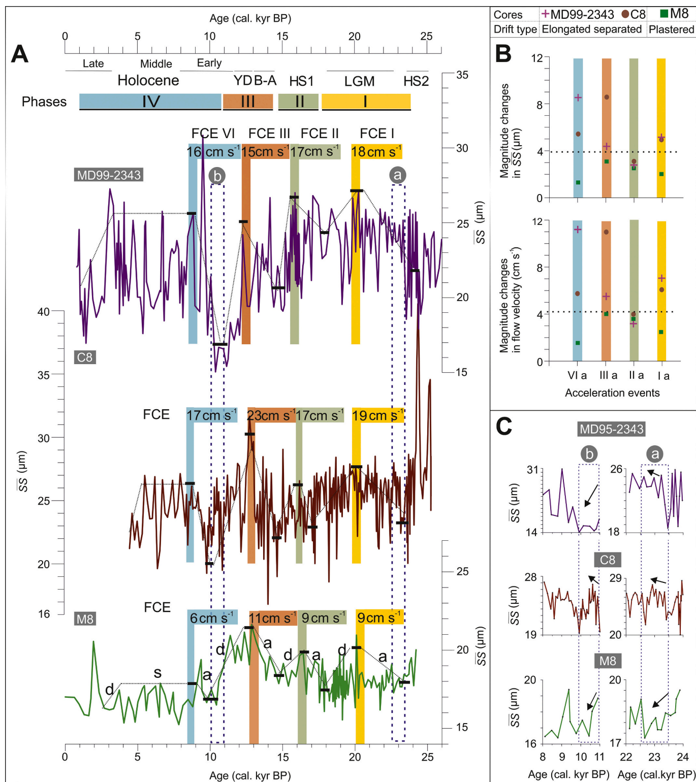
Fig. 10. Millennial scale dynamics of WMDW flow for the last 24 cal. kyr BP from the NW (core MD99–2343) to SW Mediterranean (cores C8 and M8). A) Temporal distribution of the three \overline{SS} records showing four synchronous phases (I to IV) indicating accelerations (a), deceleration (d) and steady (s) subphases and estimated paleo-velocities of the fast current events (FCE). B) Two binary plots represented by the magnitude change in \overline{SS} and in WMDW flow paleo-velocity vs the four current acceleration subphases (Ia to IVa). C) Temporal distribution of \overline{SS} for two temporal windows, 23.5–22.5 and 11–10 cal. kyr BP showing two non-synchronous events of the WMDW.
