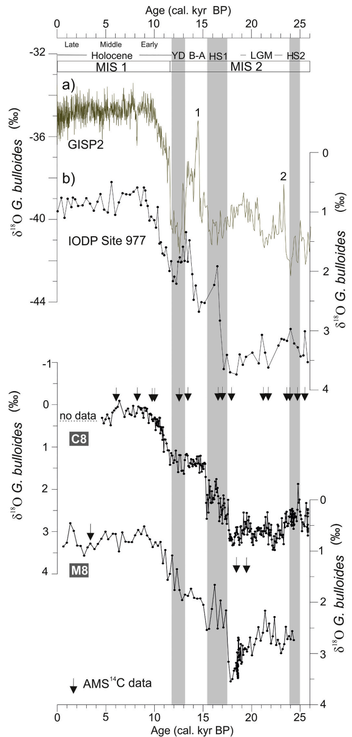
Fig. 2. Oxygen isotopic records ( \delta^{18}\text{O} ) for the last 25 cal. kyr BP for the GISP2 ice core ( Groote et al., 1993 ), IODP Site 977 ( Martrat et al., 2004 ), core C8 ( Ausín et al., 2015 ), and core M8. Black arrows refer to AMS ^{14}\text{C} data of cores C8 and M8. The gray bars indicate cold stadials (HS2 Heinrich Stadial 2, HS1 Heinrich Stadial 1, and YD Younger Dryas). LGM Last Glacial Maximum, B-A Bølling-Allerød warm period, MIS 1 and MIS 2 Marine Isotope Stages 1 and 2. Numbers 1 and 2 indicate Dansgaard-Oeschger interstadial events in the GISP2 record.
