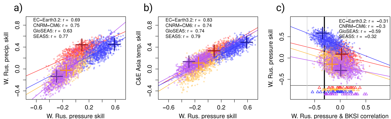
Figure 3. Scatterplots with the DJF skill relationship between (a) sea level pressure (x axis) and precipitation (y axis) in western Russia, (b) sea level pressure in western Russia (x axis) and surface air temperature in northern central and East Asia (y axis), and (c) the correlation between western Russia sea level pressure and November BKS index (x axis) and the skill in western Russia SLP (y axis). Red, yellow, blue, and purple points display values from EC-Earth3.2, CNRM-CM6-1, GloSea5, and SEAS5, respectively. All displayed r values are significantly different from 0 at the 0.05 confidence level using a one-sided T test after a Fisher transformation. The dark colored crosses represent the values from the full ensembles, while the triangles at the bottom represent the strength of the teleconnection of individual ensemble members. The black and gray vertical lines show the mean and 95% confidence interval of the correlation between ERA-Interim sea level pressure and CERSAT sea ice cover, respectively.
