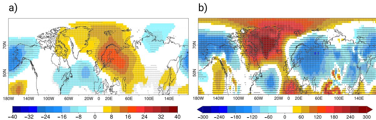
Figure 4. (a) Difference in multimodel November sea level pressure (Pa) of the top and bottom 10% random subensembles with strongest and weakest anticorrelation between DJF sea level pressure in west Russia and November BKS index, respectively. (b) Multimodel mean November sea level pressure bias (Pa). Dots indicate statistically significant values at the 0.05 confidence level using a two-sided T test.
