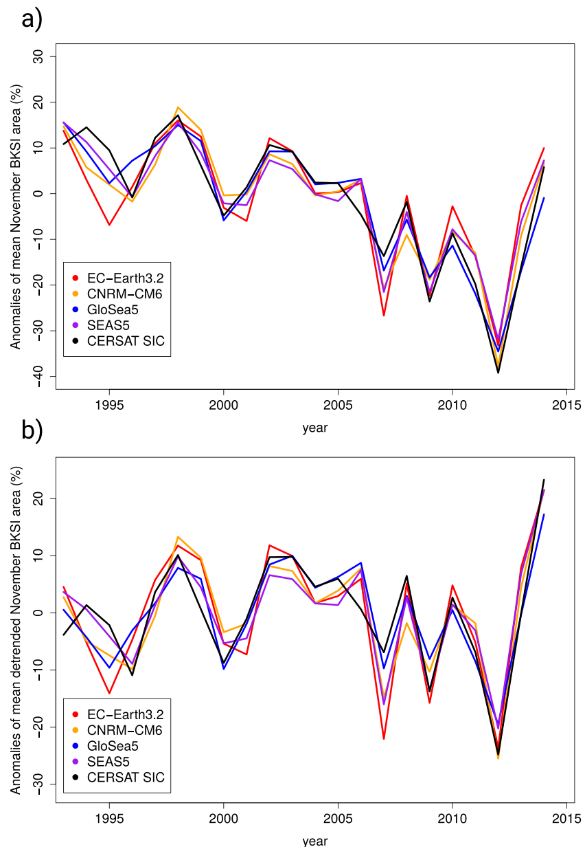
Figure 1. Sea ice cover anomalies over the Barents and Kara Seas (BKSI) in November. (a) Ensemble mean forecasts initialized every 1 November in each individual system (colors) and in the observational reference (black). (b) Same as (a) but after linearly detrending the November BKSI index.
