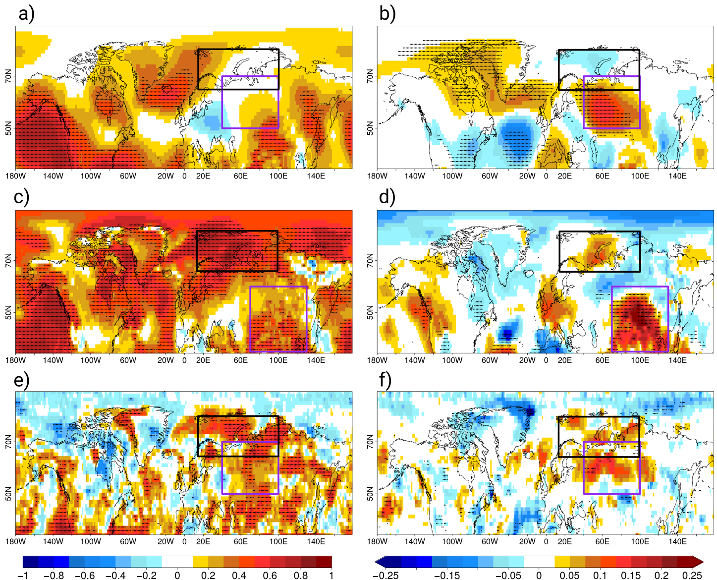
Figure 2. Skill (linear correlation) in multimodel mean DJF (a) sea level pressure, (c) surface air temperature, and (e) precipitation anomalies. Skill impact (difference in correlation between the set of forecasts with and without the November Bksi index signal) of the November Bksi cover in multimodel means of DJF (b) sea level pressure, (d) surface air temperature, and (f) precipitation anomalies. Dots indicate statistically significant values at the 0.05 confidence using a two-sided T test. Purple boxes in (a), (b), (e), and (f) represent western Russia, and northern central and East Asia in (c) and (d), which are the regions with the maximum gain in skill. The black box shows the Barents-Kara region.
