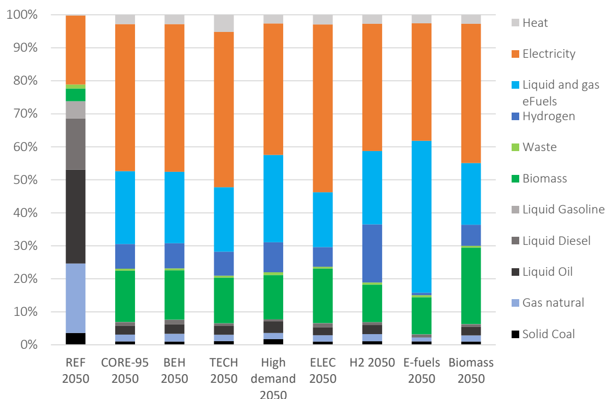
Figure 6. Final energy demand per vector (incl. industrial feedstocks, in % of total FED)
