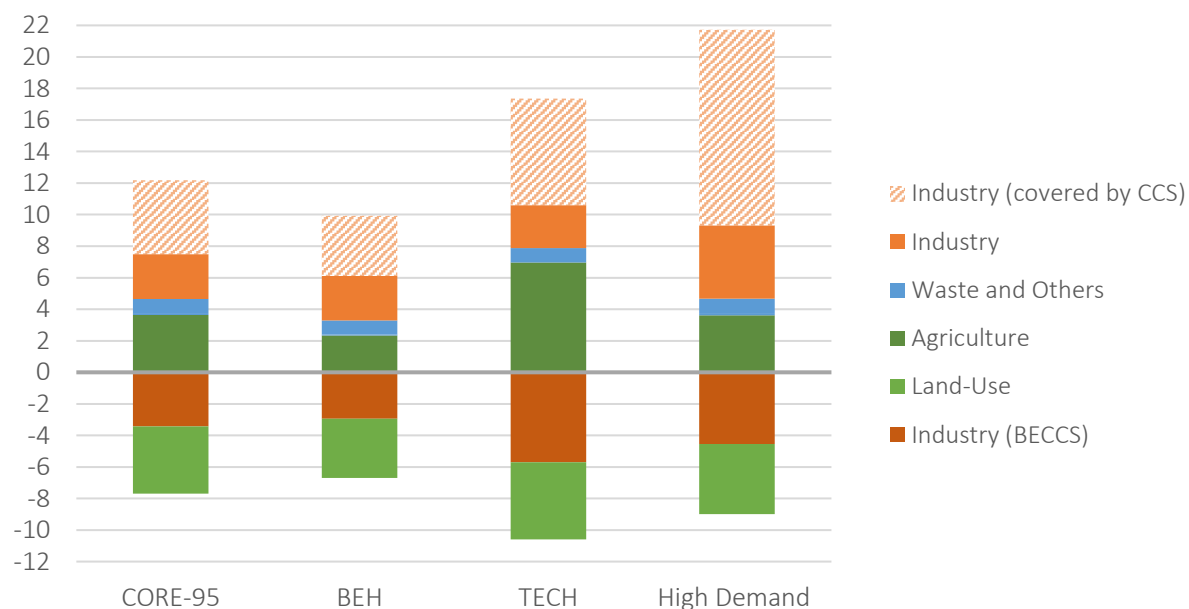
Figure 3. Emissions and removals in 2050 (in MtCO 2 e)
