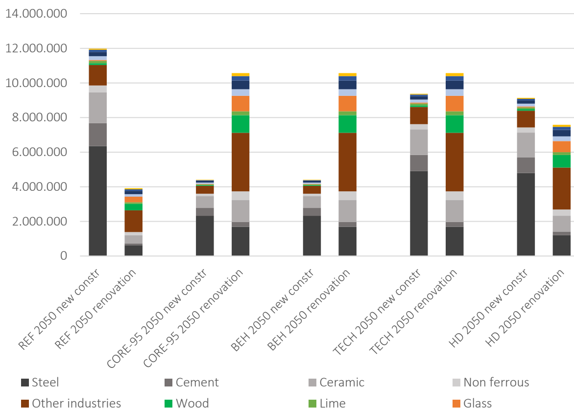
Figure 14. Material demand in the buildings sector (in tons)
