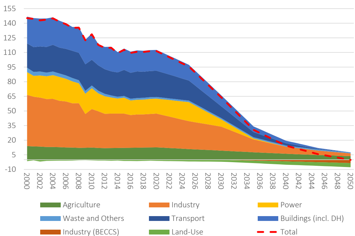
Figure 2. GHG emissions – historical and CORE-95 scenario (2000-2050, MtCO 2 e)
