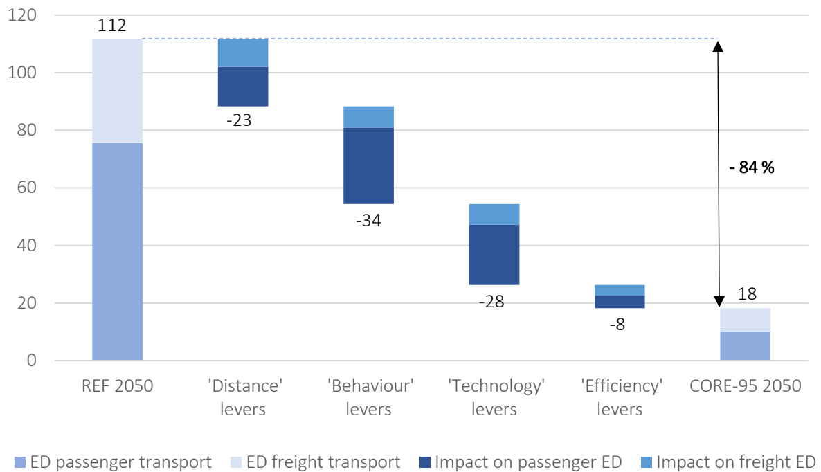
Figure 18: Contribution of different groups of levers to the reduction of energy demand in transport (in TWh) - CORE-95 scenario
