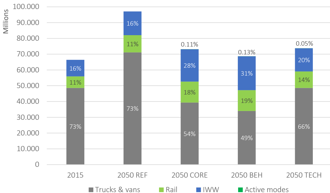
Figure 17. Freight transport demand – modal share (tkm)
