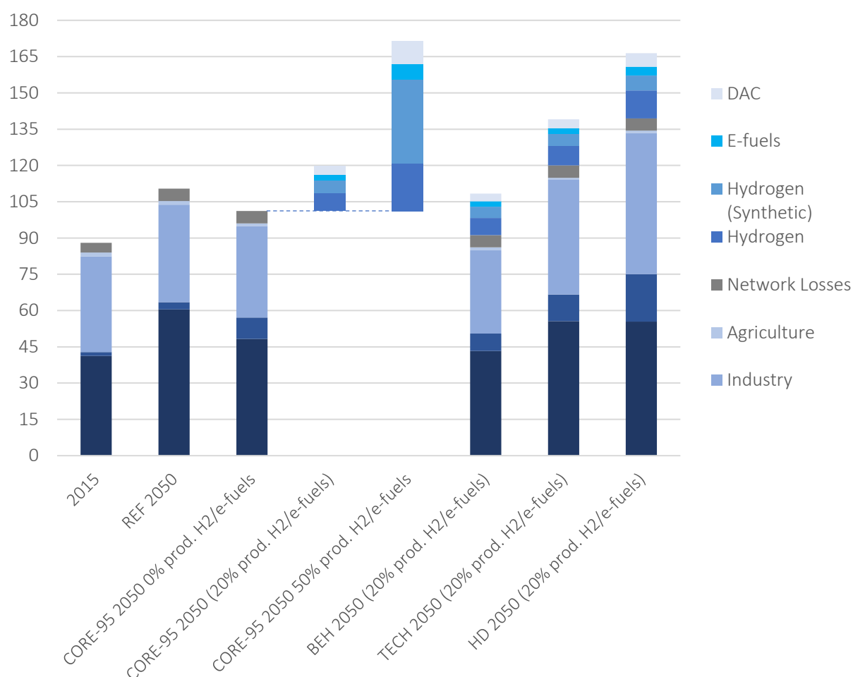
Figure 23. Total electricity demand per sector (in TWh)
