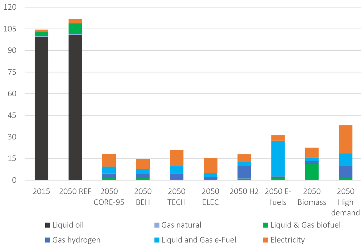
Figure 19. Total transport energy demand per vector (in TWh)
