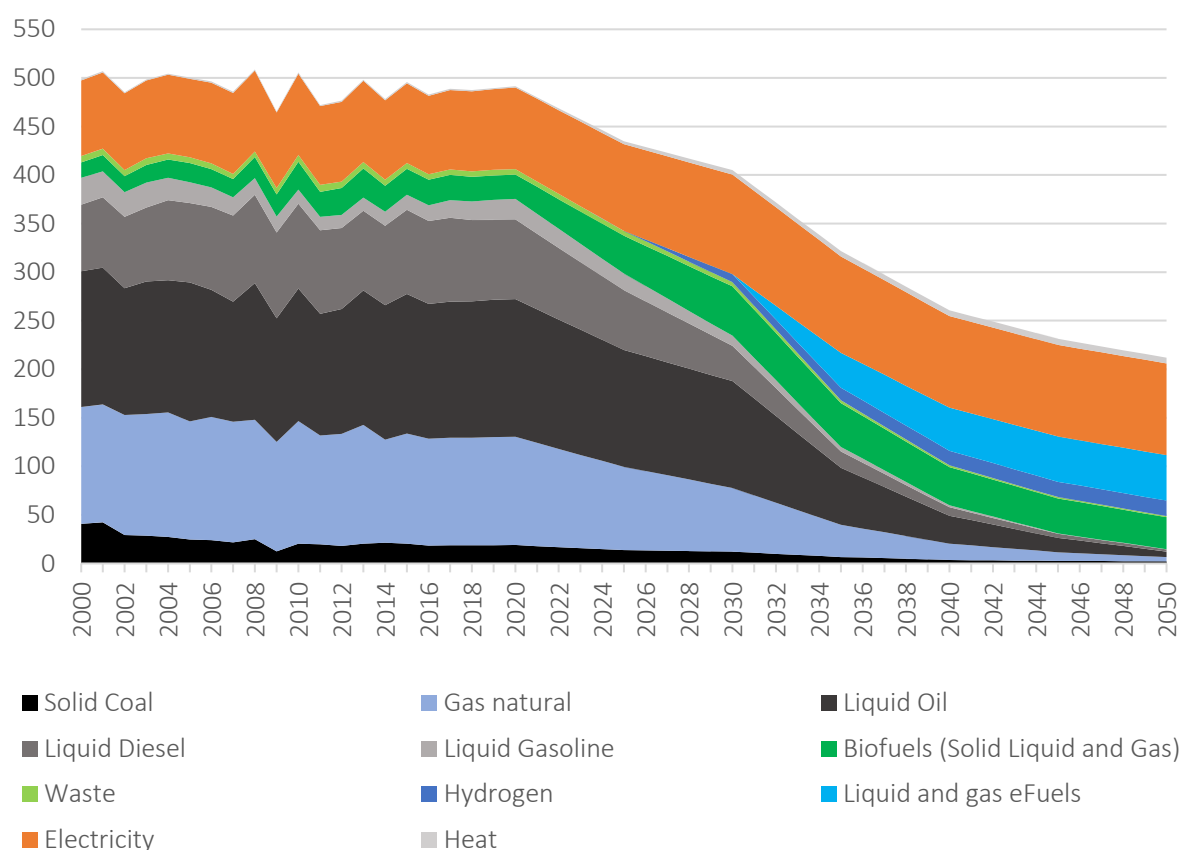
Figure 5. Evolution of final energy demand per vector (in TWh) - CORE-95 scenario
