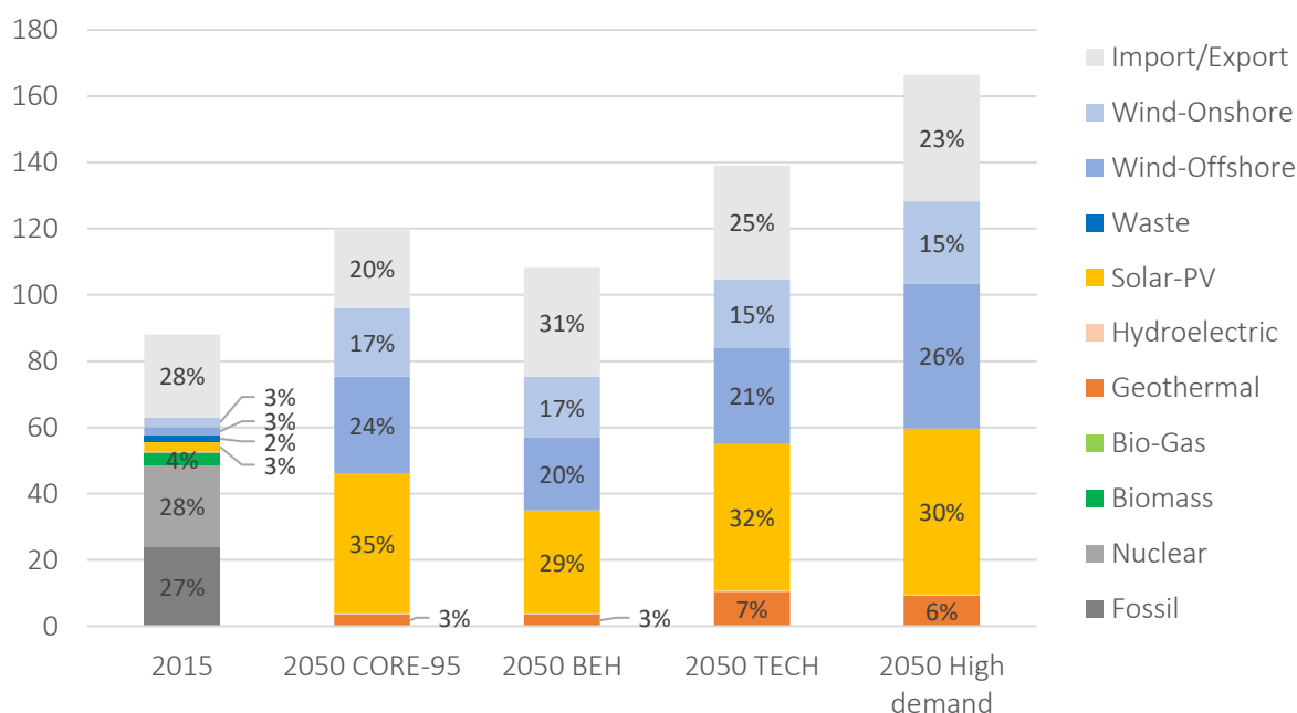
Figure 24. Electricity production (in TWh)
