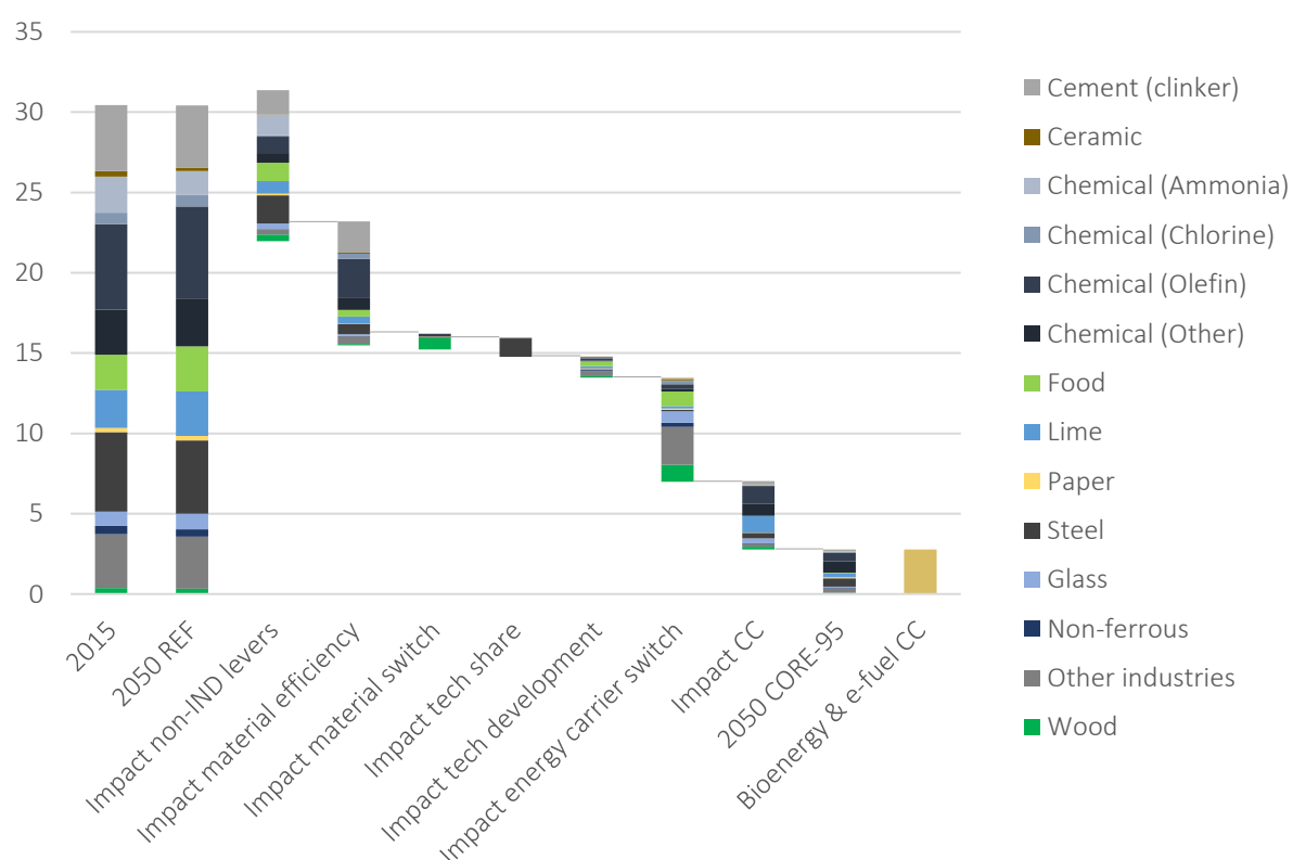
Figure 21. GHG emissions in industry – Impact of groups of levers (MtCO 2 e) – CORE-95 scenario
