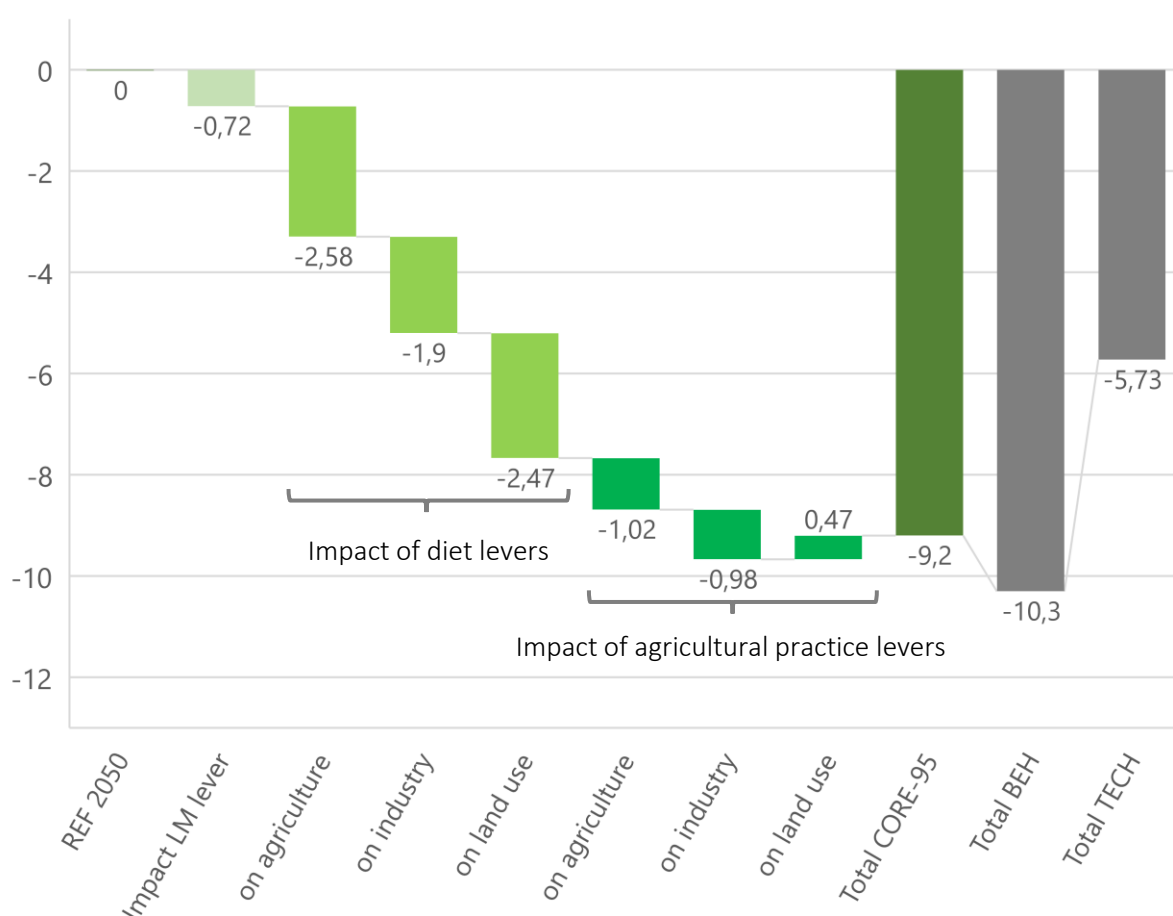
Figure 25. Impact of behavioural and agricultural practice levers on total emissions (in MtCO 2 e) as compared to REF in 2050
