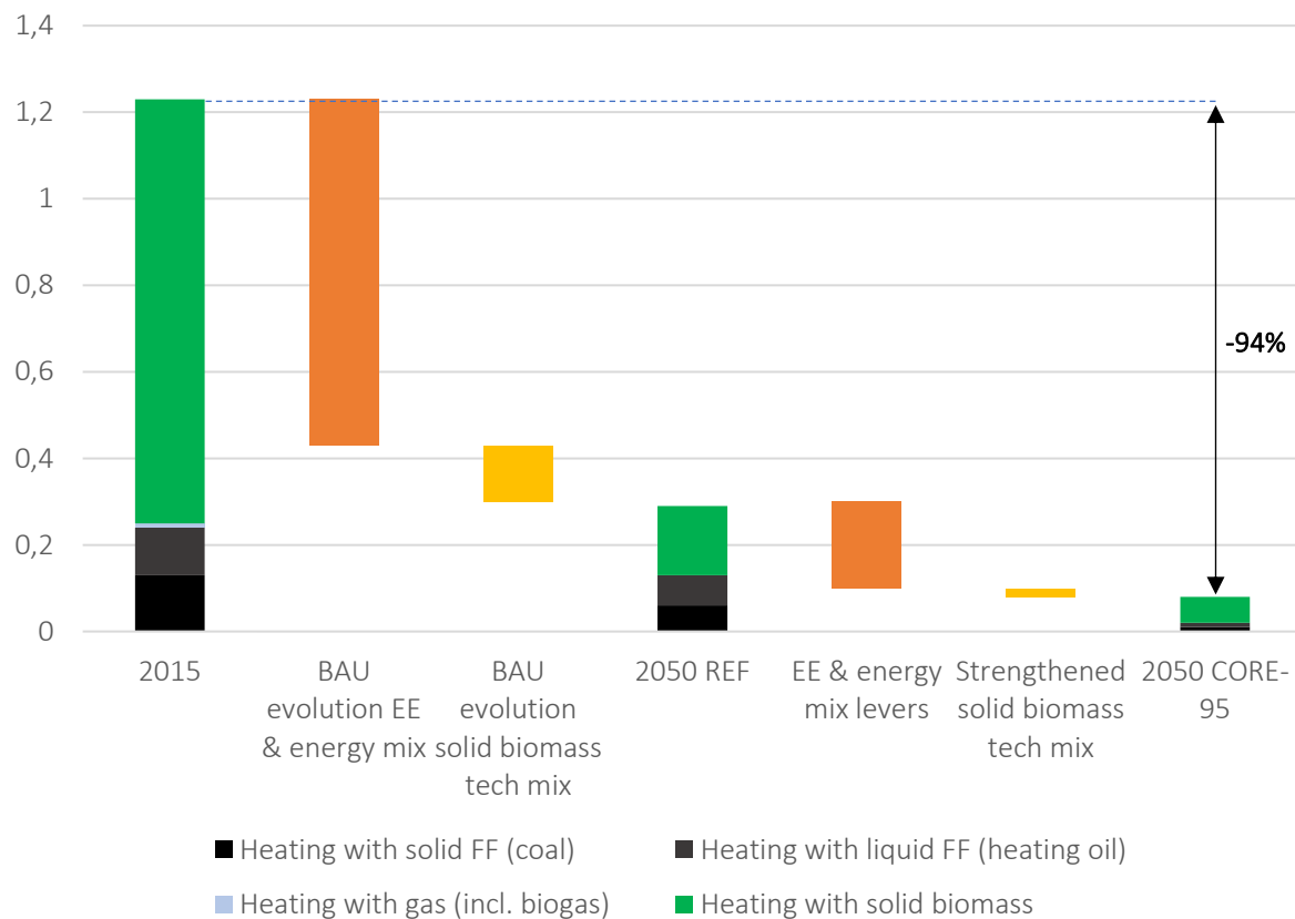
Figure 27. Emissions of air pollutants (in \mu\text{g PM}_{2.5}\text{eq/m}^3 ) for heating buildings
