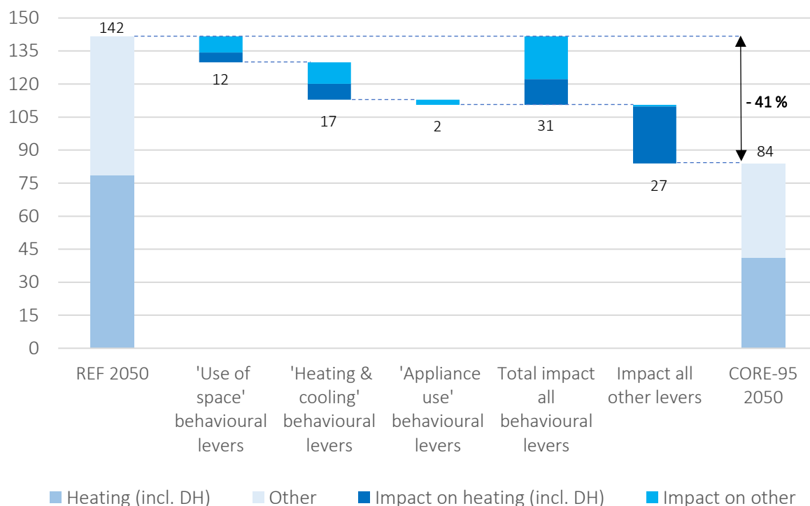
Figure 11. Energy demand per end-use in the buildings sector (in TWh) - Impact of behavioural and other levers
