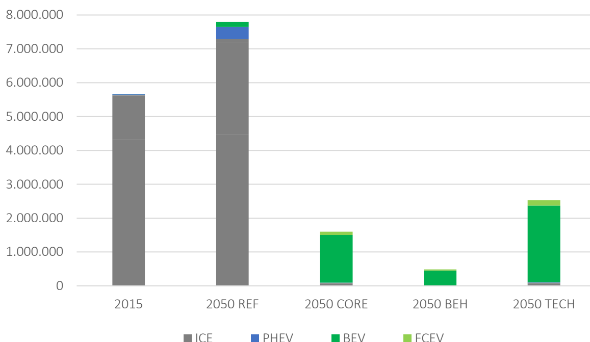
Figure 16. Number of cars by type
