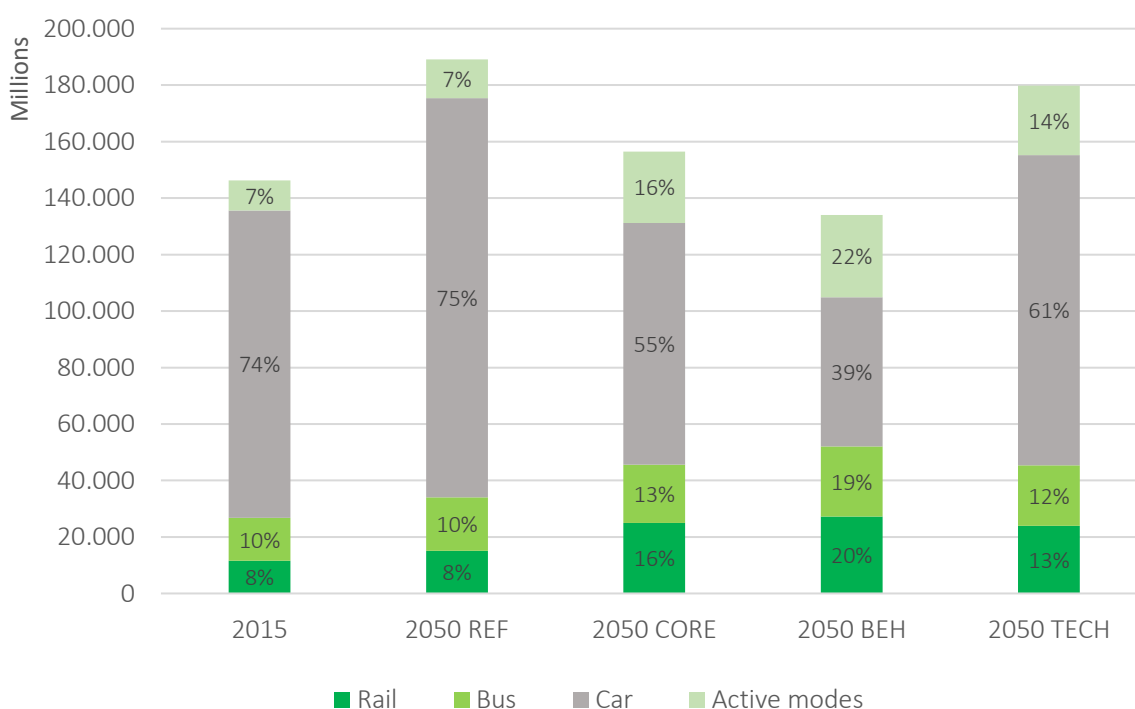
Figure 15. Total passenger transport demand (pkm) - modal share
