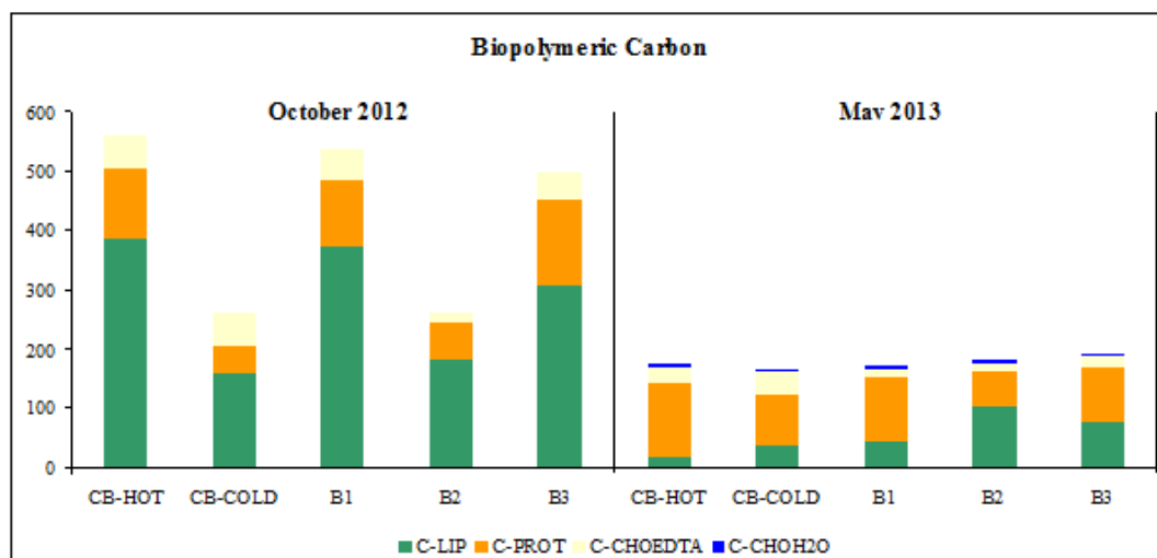
Figure 31: Biopolymeric Carbon concentration during the October 2012 and May 2013 campaigns as sum of protein (C-PROT), lipids (C-LIP), EDTA extractable carbohydrates (C-CHOEDTA) and water soluble carbohydrates (C-CHOH 2 O).
