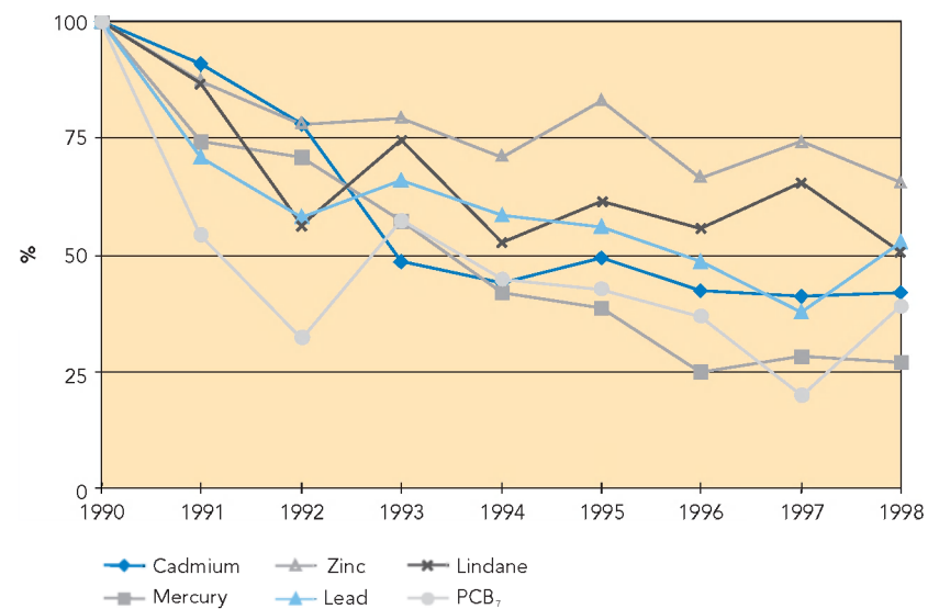
Figure 17 Change in average concentrations in rivers flowing into the North-East Atlantic including the North Sea in the period 1990–98 (average concentration in 1990 is 100 %)
