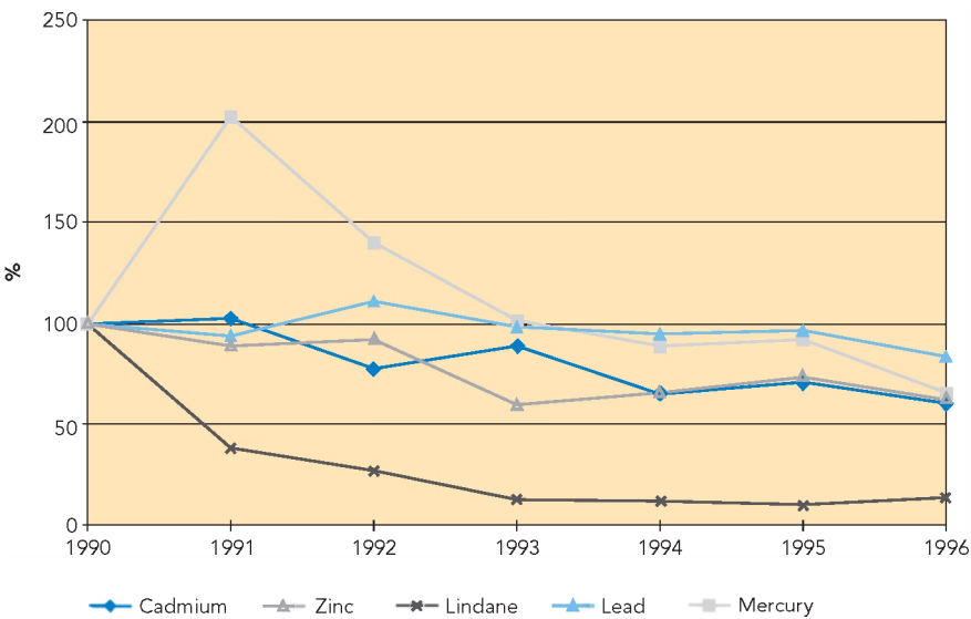
Figure 21 Change in concentrations of hazardous substances in the blue mussel in the North-East Atlantic including the North Sea in the period 1990–96 (concentration in 1990 is 100 %)
