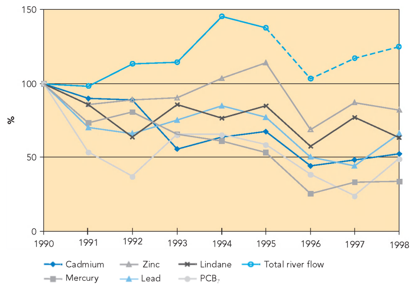
Figure 16 Change in loads (sum of direct and riverine inputs) of hazardous substances into the North-East Atlantic including the North Sea in the period 1990–98, and total river flow (input of each substance and total river flow in 1990 is set at 100 %)
