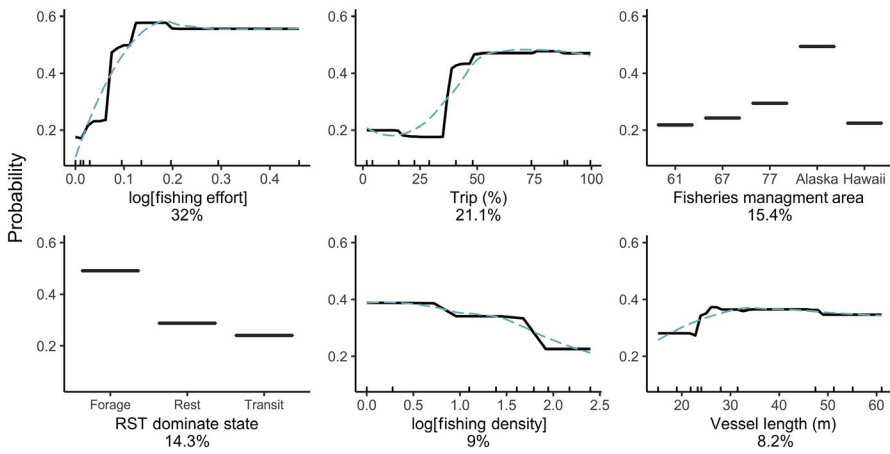
FIGURE 2 Boosted Regression Tree (BRT) partial dependency plots for the predictor variables contributing to LAAL-vessel associations with the model contribution percentage. Panels show the effect of each variable on the probability while fixing other variables at their mean. The functional (black) and smoothed (blue-dashed) response curves are shown. Rug plots show distribution of values, in deciles. Plots were constructed with ‘pdp’ (Greenwell, 2017)
