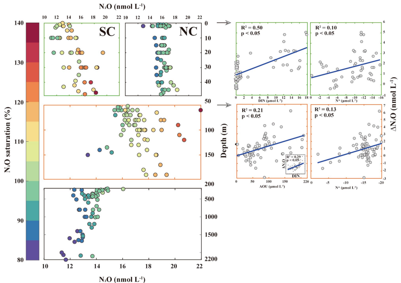
Figure 2. Vertical distribution of N_2O measured in the WAO water column during the summer of 2017 with saturation levels ( N_{2O_{\text{sat}}}(\%) = (N_{2O_{\text{measured}}}/N_{2O_{\text{eq}}}) \times 100 ; blue to red gradient color bar). Based on the vertical composition of water masses in the study area (surface, Pacific summer water and fresh water; intermediate, Pacific Winter Water; and deep areas, Atlantic Water and Arctic Bottom Water), we represent the vertical N_2O distribution by dividing into three layers (i.e., surface, 0–50 m; intermediate, 50–200 m; and deep layer, 200–2200 m). To show contrasting values associated with saturation levels (%), the surface layer is shown separately for SC and NC. To investigate the potential sources of biogeochemically derived N_2O ( \Delta N_2O ) production, the figures on the right-hand side show the correlations of \Delta N_2O with DIN and N^* in the surface layer of the SC (green color boxes), and with AOU and N^* in the intermediate layer (orange color boxes), including statistical information ( R^2 and p values). The inset shows the correlation between \Delta N_2O and DIN in the intermediate layer. Note that this figure was generated using MATLAB program (ver. R2019b and www.mathworks.com ).
