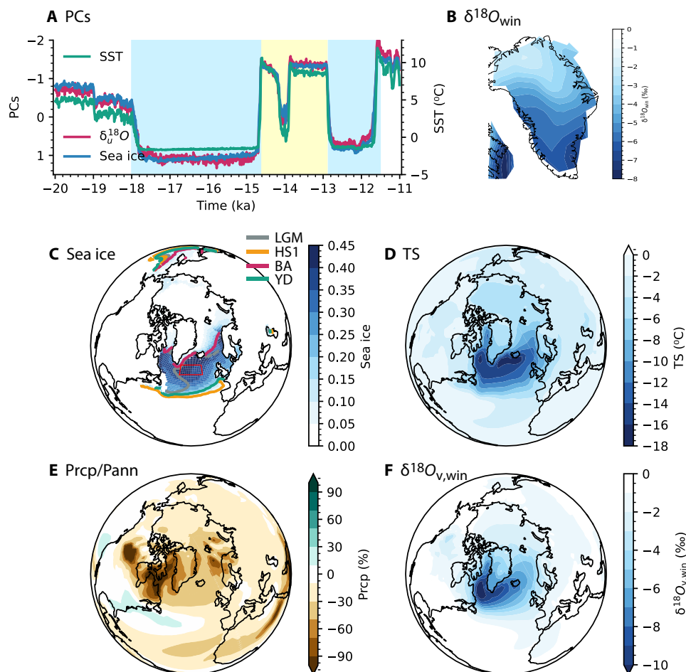
Fig. 3. Water isotope–climate–sea ice coherence in winter derived as first mode of MCA between \delta^{18}O_{win} and sea ice fraction. (A) Normalized time expansion coefficients of the first MCA mode for \delta^{18}O_{win} (red), sea ice (blue), and winter SST in the deep convection region [red box in (C)]. (B) \delta^{18}O_{win} over Greenland regressed on the normalized time expansion coefficient of sea ice. (C to F) As in (B), but for sea ice fraction, surface air temperature, precipitation change percentage (Prcp) normalized by LGM climatology, and winter column weighted water vapor \delta^{18}O_{v,win} . Regression fields at 99% ( P < 0.01 ) confidence level in two-tailed Student's t test are plotted. In (C), the curves correspond to sea ice margin as the 15% sea ice fraction in the ocean at different periods (see legend). In (F), the column water vapor \delta^{18}O_{v,win} is weighted by the moisture in each layer. Prcp, Precipitation.
