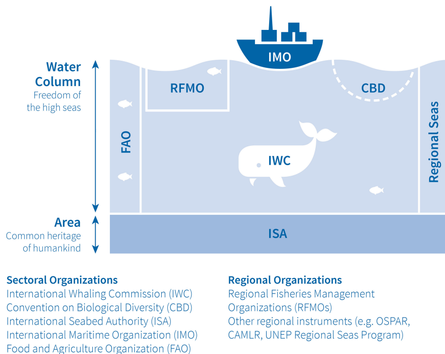
FIGURE 1 | Patchwork of sectoral and regional organizations in ABNJ.
