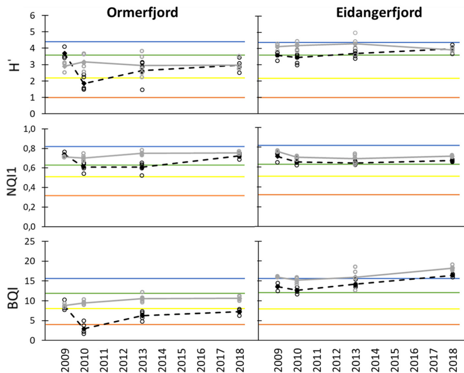
Fig. 6. Benthic indices for the various fields over time (2009–2018) (Grenland fjords). AC site = black, reference site = grey. Filled symbols show the mean value, while the empty symbols show the values for each replicate. H' = Shannon-Wiener diversity index, NQI1 = Norwegian Quality Index, BQI (Benthic Quality Index). The coloured lines show upper range of ecological classes; orange = poor, yellow = moderate, green = good, and blue = high.
