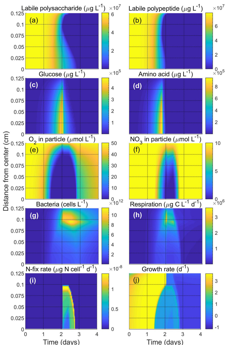
Fig. 2 Dynamics inside a particle of radius 0.125 cm with time. a Labile carbohydrate, b labile polypeptide, c glucose, d amino acid, e O_2 in particle, f NO_3^- in particle, g bacterial abundance, h respiration rate, i N_2 fixation rate, and j growth rate are shown along the particle radius over time. Parameters and concentrations of surrounding factors are taken from Table S1.
