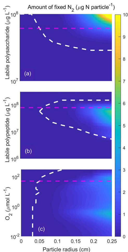
Fig. 4 Effects of particle size, O_2 , and initial polysaccharide and polypeptide concentrations on N_2 fixation rates. The total amount of fixed N_2 per particle as a function of particle radius and initial labile polysaccharide (a), initial labile polypeptide (b), and surrounding O_2 concentration (c). The white dashed line separates regions of occurrence and non-occurrence of N_2 fixation ( N_{\text{fix}} > 10^{-3} \mu\text{g N particle}^{-1} ). The horizontal magenta dashed lines indicate the base value for other plots, e.g., in (a), magenta dashed line represents the level of polysaccharide concentration in b and c. The chosen concentration ranges corresponds to those in natural particles 60,81 .
