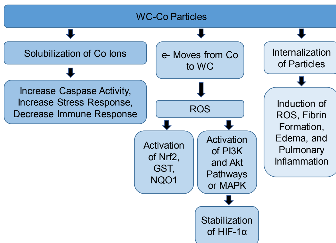
Figure 2. Summary of the proposed mechanisms of tungsten carbide-cobalt (WC-Co) toxicity. Akt: protein kinase B; GST: glutathione S-transferase; HIF-1 \alpha : hypoxia inducible factor 1- \alpha ; MAPK: mitogen-activated protein kinase; NQO1: NADPH dehydrogenase quinone 1; Nrf2: nuclear factor erythroid 2-like factor 2; PI3K: phosphatidyl inositol 3 kinase; ROS: reactive oxygen species.
