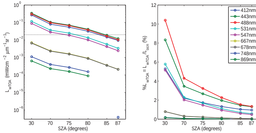
Figure 3.5 Radiance emerging from the sea that reaches the TOA, as defined by Equation 3.10, for several values of the solar zenith angle from 30° to 87°, and b) the percentage contribution of water signature to the TOA. The dashed line in a) is the accepted atmospheric correction algorithm uncertainty.
