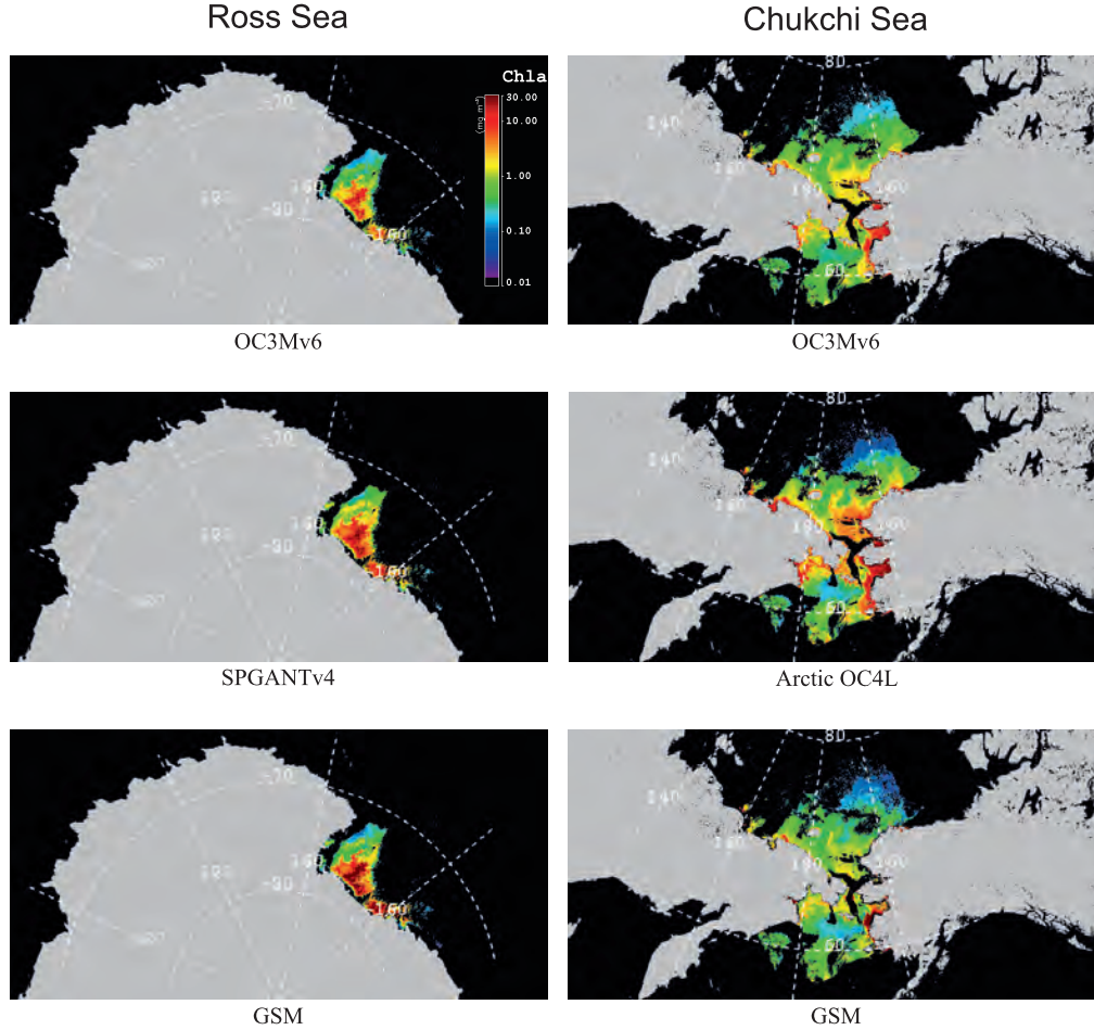
Figure 4.6 Projections of MODIS-Aqua false-colour images for two scenes from Figure 4.4, the Ross Sea and the Chukchi Sea, in which surface Chla is computed with three different algorithms; the OC3Mv6 algorithm, a regional algorithm, and the GSM. The colour bar scale for all images is depicted in the top left panel.
