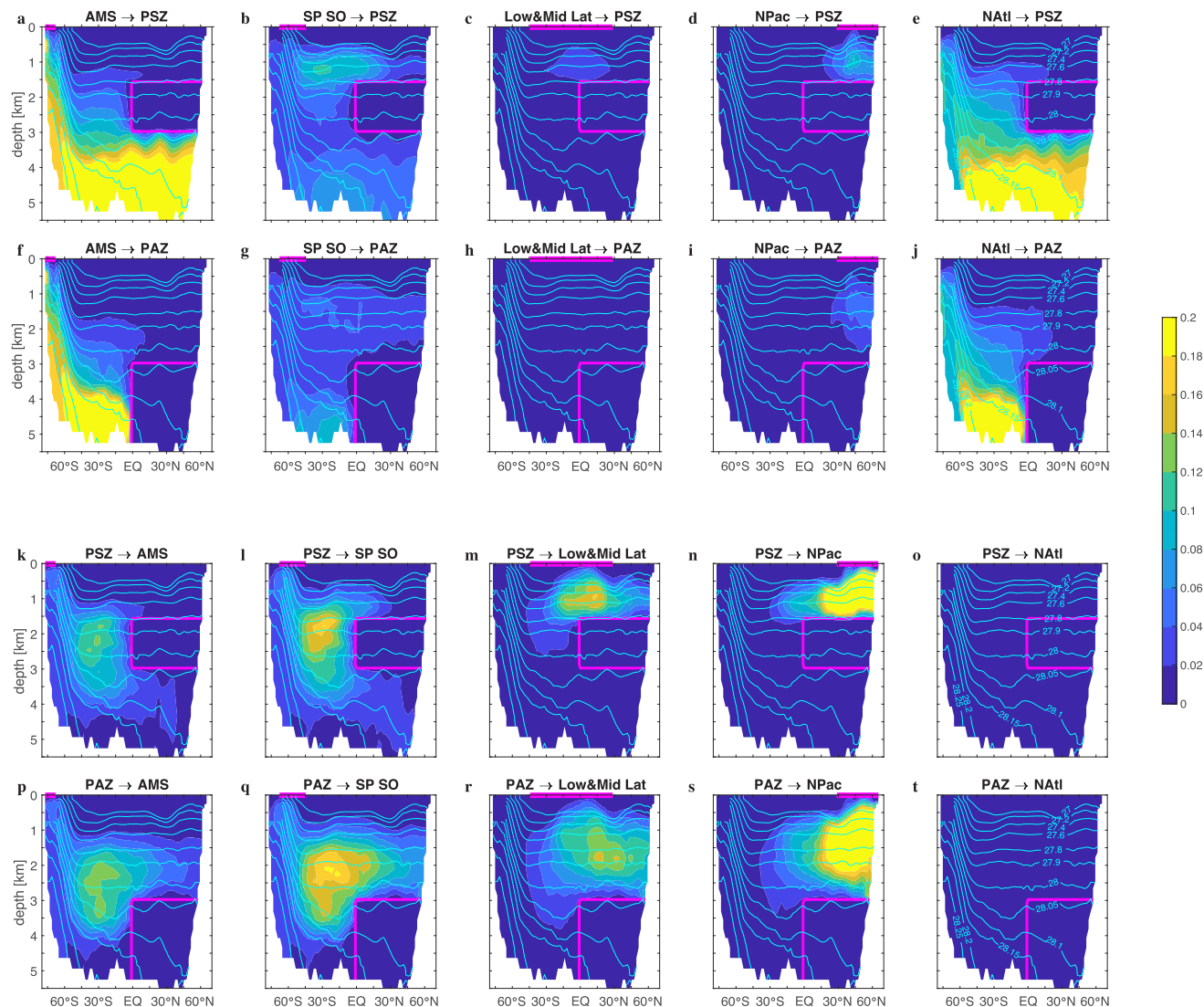
Fig. 5 Pacific zonal mean path densities. Pacific zonal averages of the surface-to-interior path density (a–j) and of the interior-to-surface path density (k–t). (The path density is the dimensionless local fraction of water in origin-to-destination transit – see Methods.) Surface origin or destination regions as indicated in the titles and defined in Fig. 4a: Antarctic marginal seas (AMS), subpolar Southern Ocean (SP SO), low and mid latitudes (Low&Mid Lat), the northern Pacific (NPac), and the northern Atlantic (NAtl). The magenta outlines indicate the Pacific Shadow Zone (PSZ) or the Pacific Abyssal Zone (PAZ) and the part of the surface regions within the Pacific, while the cyan contours are Pacific zonal mean neutral density ( -1000 ) in units of \text{kg m}^{-3} . A generic feature of the A \rightarrow B path density in the presence of diffusion is that it goes to zero close to A and close to B, where most water undergoes either A \rightarrow A or B \rightarrow B return trips 72 .
