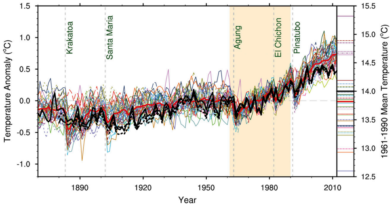
Fig. 1. Estimates of global surface temperature anomaly from model integrations performed in support of the fifth phase of the coupled model intercomparison project (CMIP5). Here, the observed anomaly (black) is estimated relative to the observed climatology, while the model anomalies are estimated relative to each model's estimate of climatology (rather than the multimodel ensemble mean estimate of climatology). This has the implicit effect of removing each model's individual climatological bias against observations. The range of uncorrected model temperatures for the period 1961 to 1990 is shown in a small bar to the right of the figure. While uncertainty in observational estimate of absolute temperatures is about 0.5 °C, uncertainty in the anomalies is much smaller. As such, the spread in model anomalies relative to the multimodel ensemble mean is larger than the observed trend in the anomalies and much larger than the uncertainty in the observed anomalies. Adapted with permission from ref. 13.
