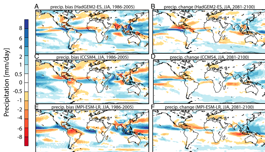
Fig. 3. A, C, and E show the systematic error of the 3 CMIP5 models in Fig. 2 for June, July, and August (JJA) mean precipitation (based on GPCP observational data) computed using ensemble integrations and observations for the same period as in Fig. 2. B, D, and F show the same 3 models' response to climate change forcing based on differences between ensemble integrations for the same period and scenario as in Fig. 2. The same scale is used for A–F. There are widespread regions where the systematic error exceeds the climate change signal (in some regions by more than a factor of 20).
