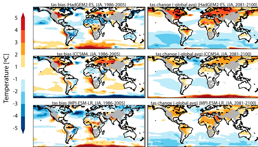
Fig. 2. The left-hand column shows the systematic error of 3 of the leading CMIP5 models for June, July, and August (JJA) mean surface air temperature (tas) computed using ensemble integrations and observations for the period 1986 to 2005. The right-hand column shows the same 3 models' regional temperature response to climate change forcing (computed as the departure from the global mean) based on differences between ensemble integrations for the period 2081 to 2100 following the RCP8.5 scenario and the period 1986 to 2005. The same scale is used for both columns. There are widespread regions where the magnitude of systematic error is comparable with or exceeds the magnitude of the climate change signal.
