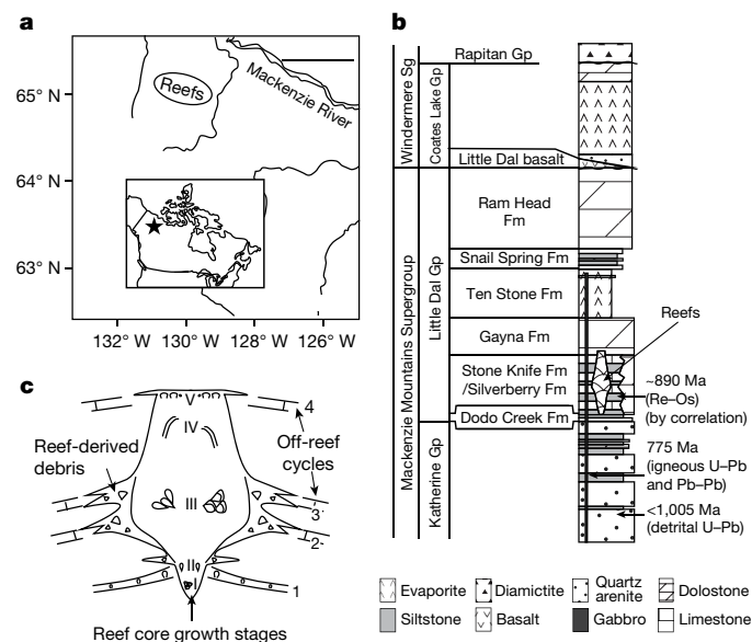
Fig. 1 | Geographic and stratigraphic location of the study material.
