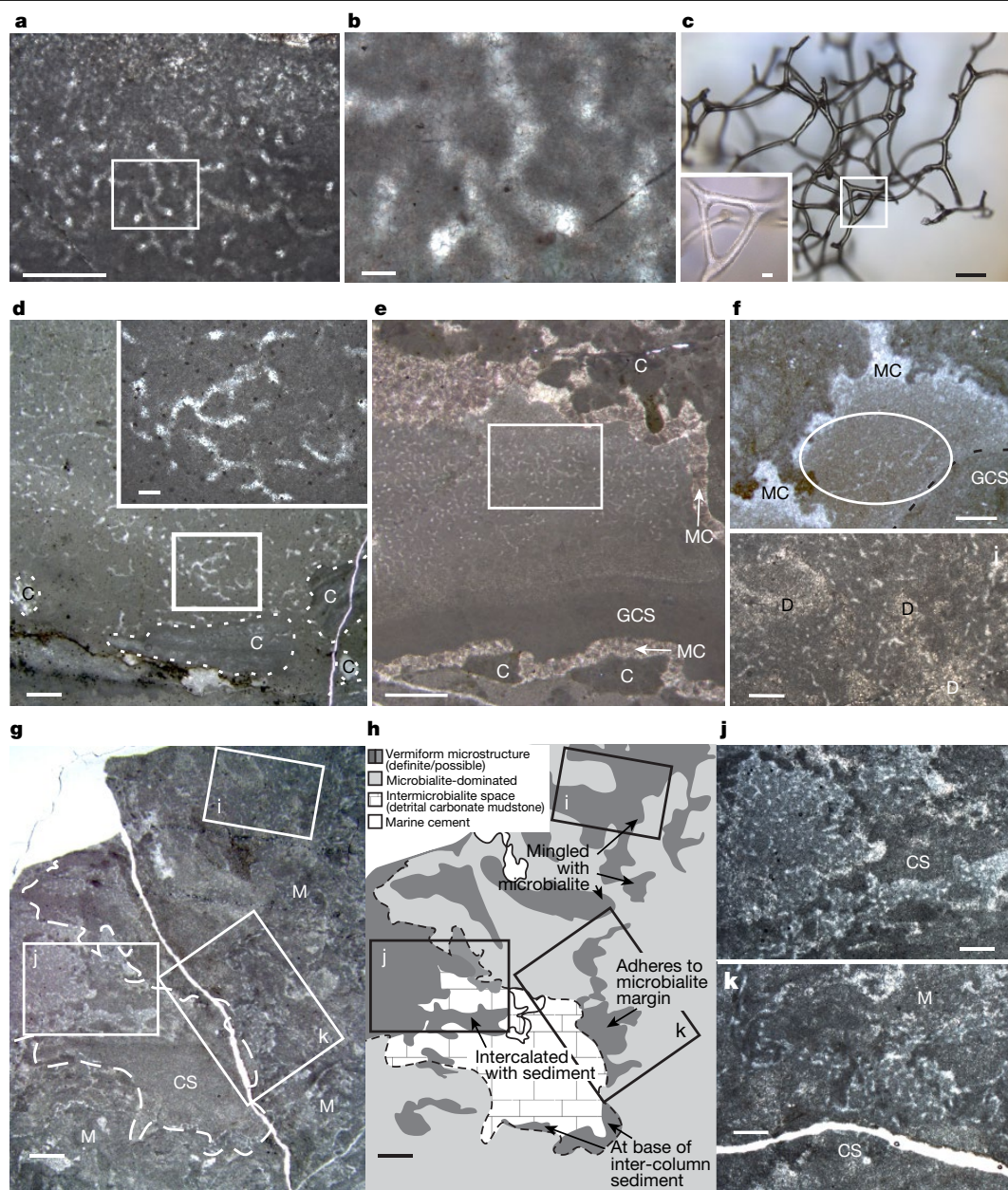
Fig. 2 | Characteristics and distribution of Little Dal vermiform microstructure in stratigraphically oriented 30- \mu m-thick thin sections.
