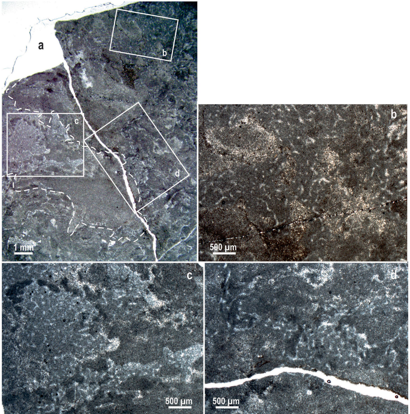
Extended Data Fig. 4 | Associations of vermiform microstructure, micritic microbialite columns and detrital sediment in microfacies i and iiia.
