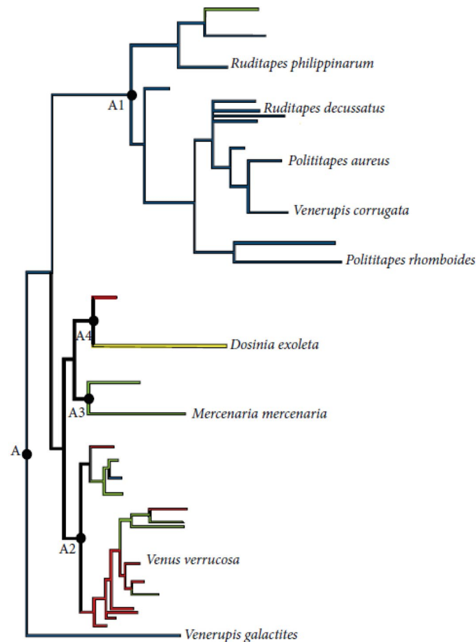
Figure 2. Phylogenetic tree proposed by 93 . Modified from 5 .
