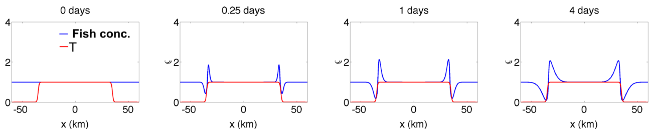
Figure 6. Time evolution of the fish concentration as reported in Fig. 5. This time, the plateau width has been set to 70 km.
