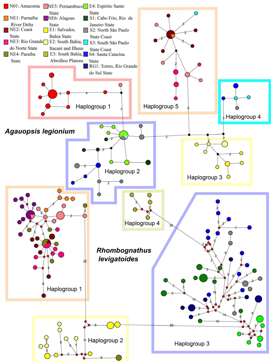
FIGURE 2 Minimum spanning network showing relationships among haplotypes of Agauopsis legionium and Rhombognathus levigatooides ; different populations are color-coded. The number of mutational steps (>1) along the edges is indicated. Circles representing haplotypes are scaled to their frequencies. Haplogroups are referred to in the text
