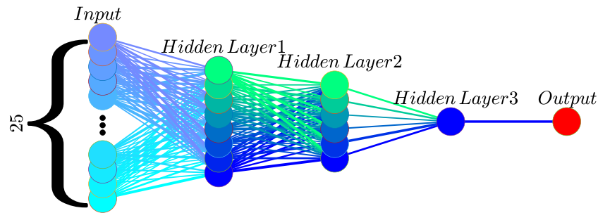
Figure 3. The neural network architecture used in this study, which is made of an input layer, an output layer, and three hidden layers. The symbols are the same as those in (1). The matrices/vectors \mathbf{w}_i and \mathbf{b}_i ( i = 1, 2, 3, 4 ) are obtained through training. To predict the El Niño Modoki Index (EMI) at month/step n , \text{EMI}(n) , find the first 25 principal components of [\text{SSN}(n - 600), \text{SSN}(n - 599), \dots, \text{SSN}(n - 265)]^T , a column vector with 336 entries, and form the input vector \mathbf{x} . The final output y is the predicted \text{EMI}(n) . Iterating on n , we can get a prediction of EMI for any target time interval. (Figure generated with MATLAB, Version 6.5. http://www.mathworks.com/ ).
