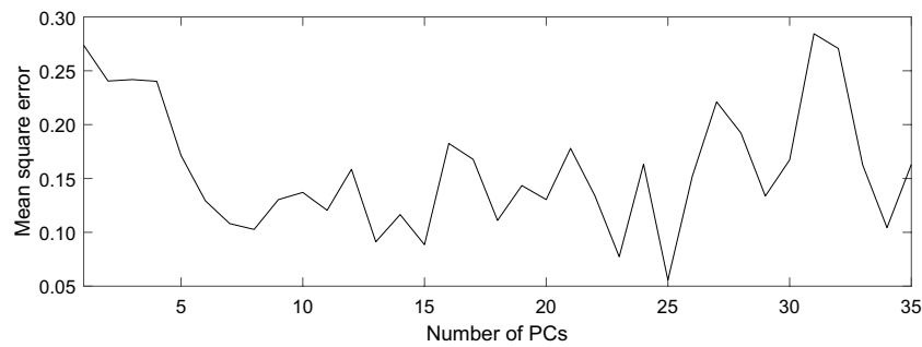
Figure 6. Mean square error for the neural network prediction as a function of number of principal components. (Figure generated with MATLAB, Version 6.5. http://www.mathworks.com/ ).
