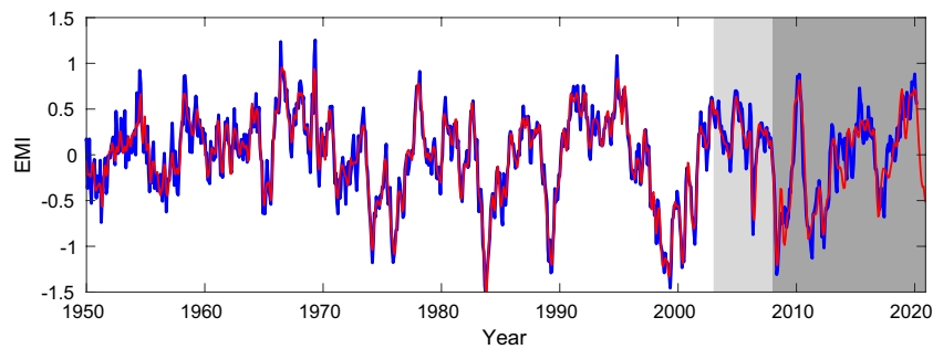
Figure 4. Prediction of the El Niño Modoki index based solely on the sunspot numbers 22–50 years ago with the back propagation neural network algorithm. The EMI is in blue, while the predicted index is in red. Lightly shaded is the period over which the validation set is formed, and the period with dark shading is for prediction. (Figure generated with MATLAB, Version 6.5. http://www.mathworks.com/ ).
