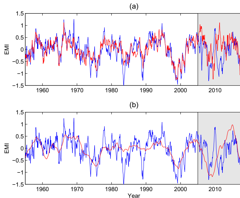
Figure 2. Prediction of the El Niño Modoki index based solely on the sunspot numbers 22–50 years ago with a simple linear regression model. (a) The SSN series are bandpass filtered with the annual signals and the signals longer than 11 years removed. (b) Only 25 first principal components are used as inputs. The shaded period is for prediction, and the predicted index is in red. (Figure generated with MATLAB, Version 6.5. http://www.mathworks.com/ ).
