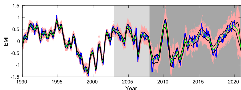
Figure 5. The 1000 predictions showing the spread of the ensemble. Overlaid are the observed EMI (blue), the mean of the realizations (cyan), and the mean plus and minus the standard deviation (black). The light shading marks the period for validation, while the darker shading marks the prediction period. (Figure generated with MATLAB, Version 6.5. http://www.mathworks.com/ ).
