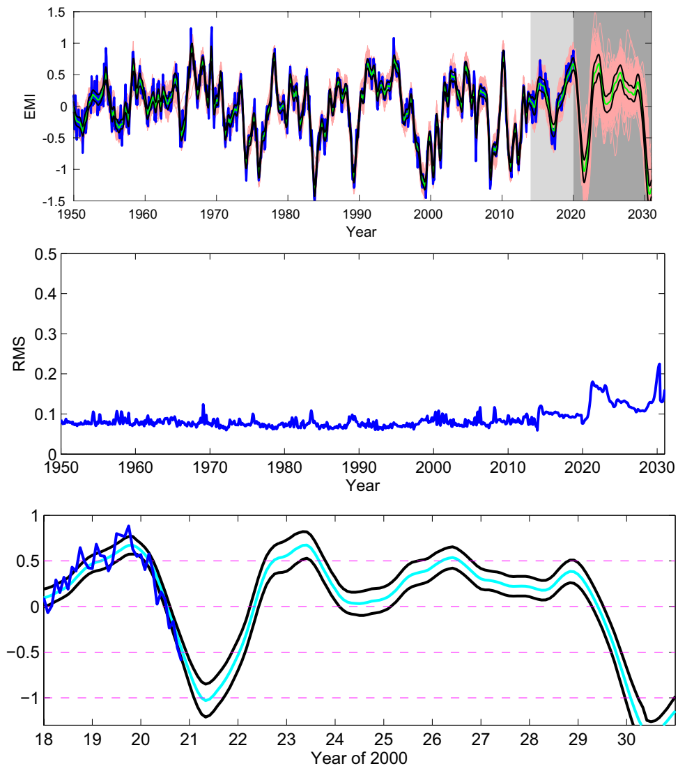
Figure 9. Top: As Fig. 5, but using a model based on series with delays from 10 through 43 years, with the time intervals forming the training set and validation set being, respectively, 01/1920–12/2013 and 01/2014–02/2020. Middle: The corresponding standard deviation around the ensemble mean. Bottom: A close-up of the prediction over 2018–2030. (Figure generated with MATLAB, Version 6.5. http://www.mathworks.com/ ).
