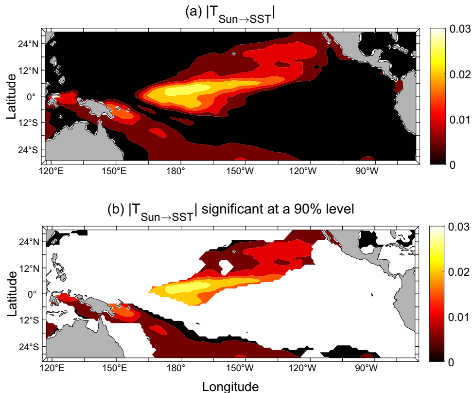
Figure 1. (a) The absolute information flow from the delayed (by 45 years) series of sunspot numbers to those of the sea surface temperature in the Pacific Ocean (in nats/month). The pattern resembles very much the El Niño Modoki mode as shown in the Fig. 2b of 6 . Here information flow means the transfer of predictability from one series to another. It is computed with Eq. (6) in “Method”. (b) As (a), but only the information flow significant at a 90% confidence level is shown. (Figure generated with MATLAB, Version 6.5. http://www.mathworks.com/ ).
