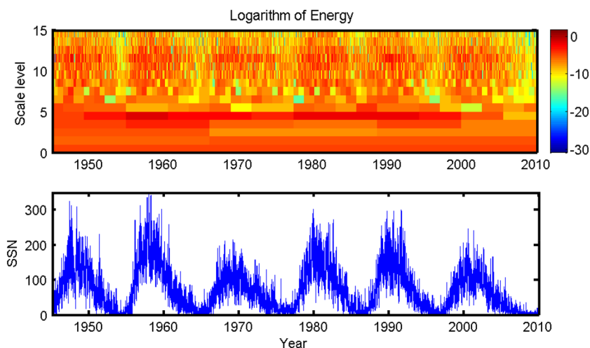
Figure 10. Daily series and orthonormal wavelet spectrum of the sunspot numbers based on the spline wavelets built in 30 . (Figure generated with MATLAB, Version 6.5. http://www.mathworks.com/ ).
