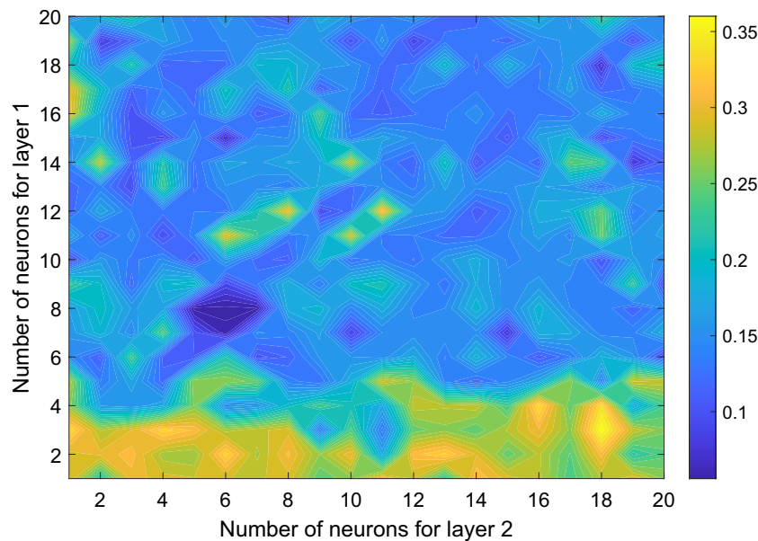
Figure 7. Mean square error as function of number of neurons. (Figure generated with MATLAB, Version 6.5. http://www.mathworks.com/ ).
