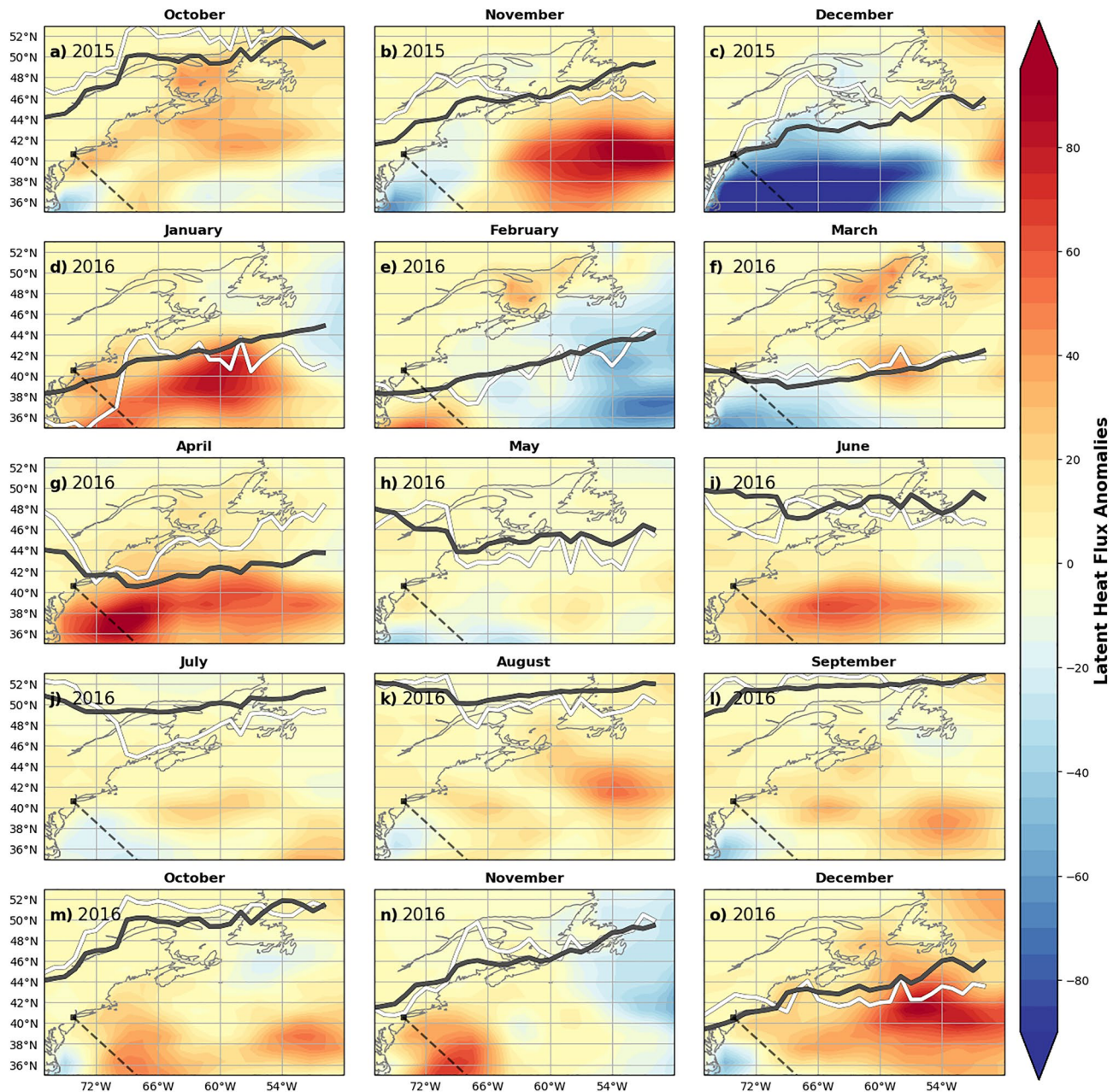
Figure 6. Latent heat flux anomaly for the 2015/16 period. Negative (positive) anomalies indicate the ocean is gaining (losing) more heat than usual for the 1986–2016 period. The thick gray line is the climatological position of the jet stream (1986–2016). The thick white line is the jet stream's latitudinal position for 2015/16. These maps were generated using Python version 2.7.5.
