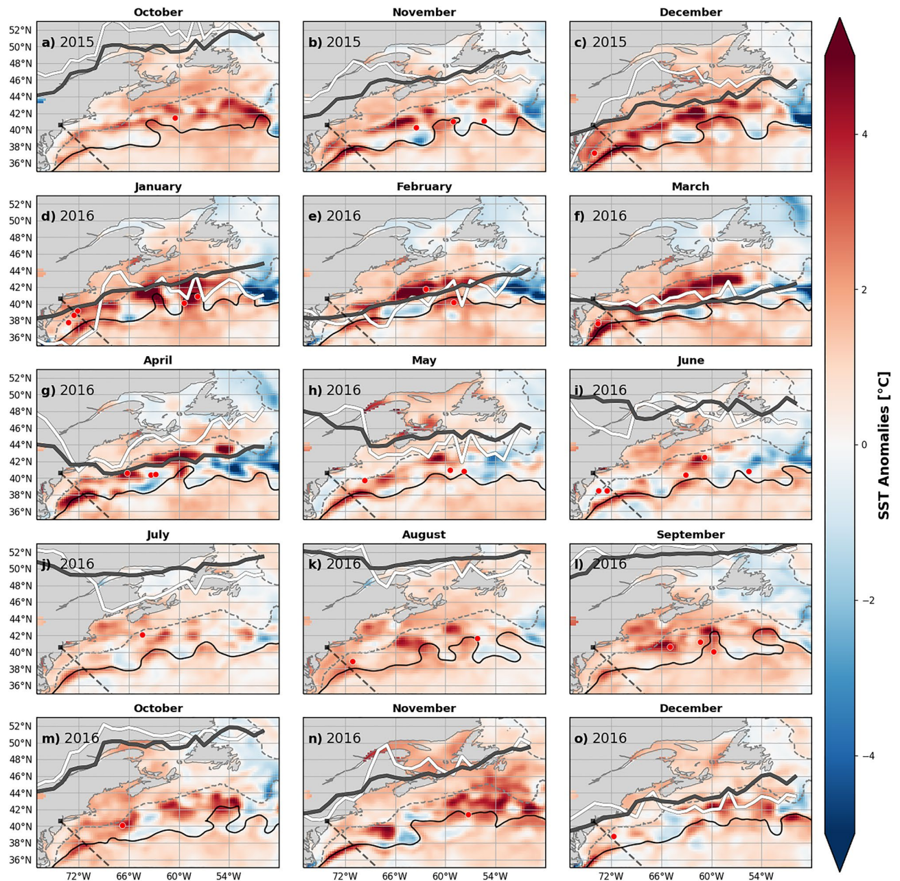
Figure 3. SST anomalies in the NWA for the 15-month period 2015/16. Black dashed line indicates the Oleander Line. Black solid curve indicates the average Gulf Stream path (based on 25 cm SSH isoline) for each month. Positions of WCRs on their date of absorption for the 15-month period are indicated with red dots. Gray dashed line is the isobath contour at 500 m. The thick gray line is the climatological position of the jet stream (1986–2016). The thick white line is the jet stream's latitudinal position for 2015/16. These maps were generated using Python version 2.7.5.
