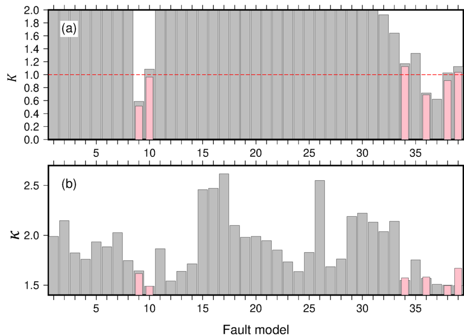
Figure 4. Histograms for (a) K and (b) \kappa for all fault models obtained with the non-dispersive and dispersive equations (gray and pink bars, respectively). The dashed red line indicates K=1 , representing a good match between the observations and predictions. The dispersive model was calculated only for fault models 9, 10, 34, 36, 38, and 39 because of computational resource limitations.
