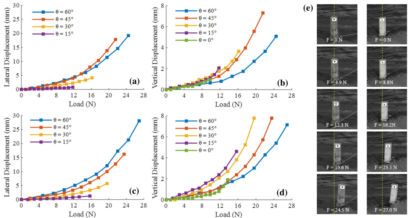
Figure 5. Lateral and vertical displacement–load curves with variables angle of circular pile (a,b) and square pile (c,d), and the failure process of circular pile (left column) and square pile (right column) with \theta = 60^\circ (e).
