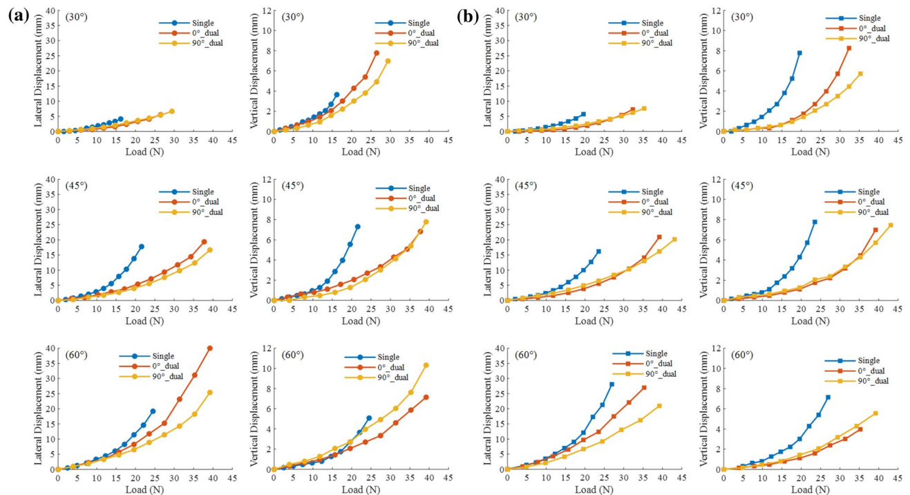
Figure 9. Lateral and vertical displacement-load curves of circular (a) and square (b) anchor piles with variables configuration.
