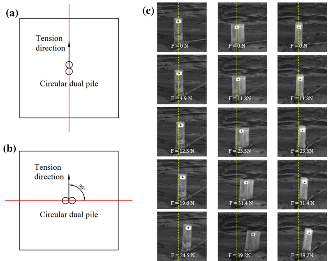
Figure 10. Different layouts of dual piles 0°_dual (a) and 90°_dual (b). Photos of the failure process of variables pile configuration (left column: circular single pile; middle column: circular 0°_dual layout; right column: circular 90°_dual layout) with \theta = 60^\circ (c).
