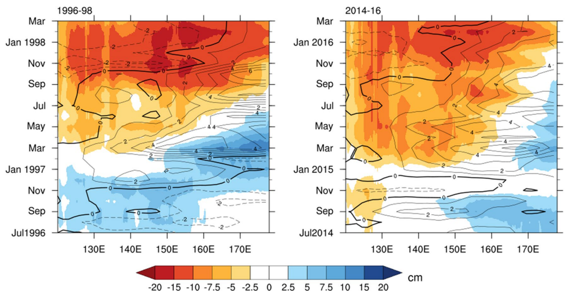
Figure 6. Time-longitude plot of BRAN sea level height (shaded, cm) and ERA-interim surface zonal wind (contours, \text{m s}^{-1} ) anomalies averaged between 5^{\circ}\text{S} and 5^{\circ}\text{N} for two El Niño events during 1996–1998 and 2014–2016, respectively. Plots are generated using the NCAR Command Language version 6.6.2 ( http://www.ncl.ucar.edu/ ).
