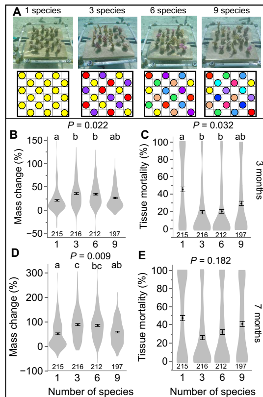
Fig. 3. Positive biodiversity effects peak at intermediate coral species richness.
