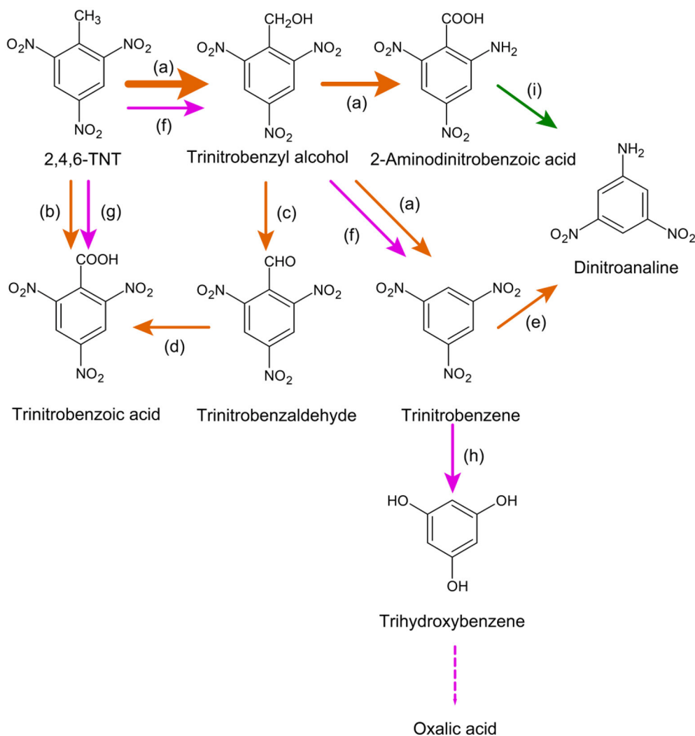
FIGURE 8 | TNT transformation and mineralization via photo- and Fenton- reaction. Symbols as in Figure 6 . References: a, Spanggord et al. (1983), Godejohann et al. (1998), Luning Prak et al. (2017), and Burlinson et al. (1979a); b, Luning Prak et al. (2017) and Burlinson et al. (1979a); c, Luning Prak et al. (2017); d, Godejohann et al. (1998), Kaplan et al. (1975), and Schmelling and Gray (1995); e, Spanggord et al. (1983) and Godejohann et al. (1998); f, Jarand et al. (2011) and Hess et al. (2003); g, Hess et al. (2003); h, Hess et al. (2003), Liou et al. (2003), and Li et al. (1998); i, Spanggord et al. (1983) and Godejohann et al. (1998).
