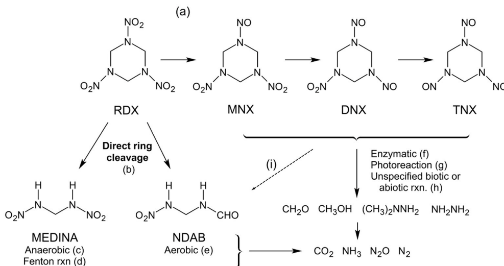
FIGURE 9 | RDX transformation and mineralization reaction pathways. HMX degradation follows identical pathways, and is not shown here for simplicity. References: a, Juhasz and Naidu (2007), McCormick et al. (1981), Van Aken et al. (2004), Hawari et al. (2001), and Sheremata et al. (2001); b, Ariyaratna et al. (2016), Halasz and Hawari (2011), Smith et al. (2015b), Liou et al. (2003), and Hawari et al. (2001); c, McCormick et al. (1981), Jackson et al. (2007), and Hawari et al. (2000c); d, Liou et al. (2003), Oh et al. (2003), and Zoh and Stenstrom (2002); e, Jackson et al. (2007) and Monteil-Rivera et al. (2008); f, Van Aken et al. (2004); g, Van Aken et al. (2004) and Bose et al. (1998); h, Ariyaratna et al. (2016), Hawari et al. (2000c), Monteil-Rivera et al. (2008), and Zhao et al. (2004); i, McCormick et al. (1981).
