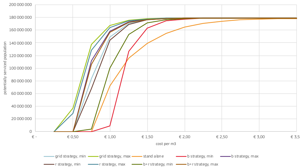
Figure 5.24 costs of water production under different assumptions in the Mediterranean.
