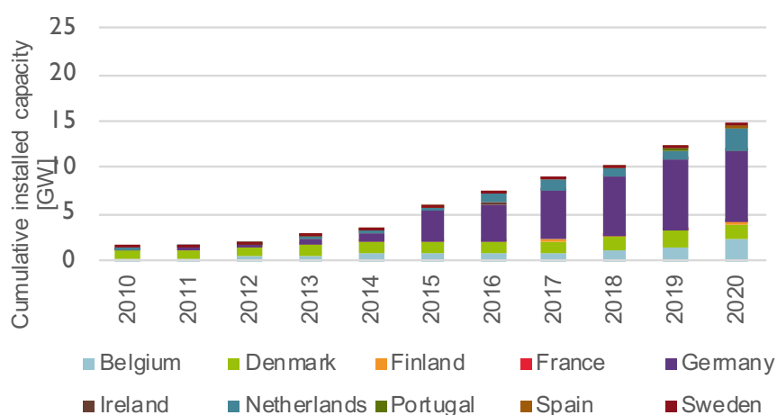
Figure 4.12 EU offshore wind energy installed capacity, MW
