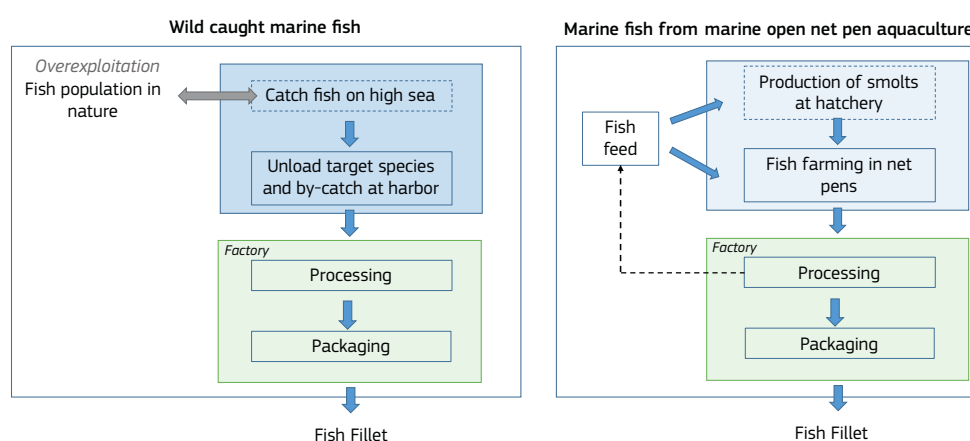
Figure 6.10 Life cycle stages of fish fillet from marine fish either from wild caught or from open net pen aquaculture.
