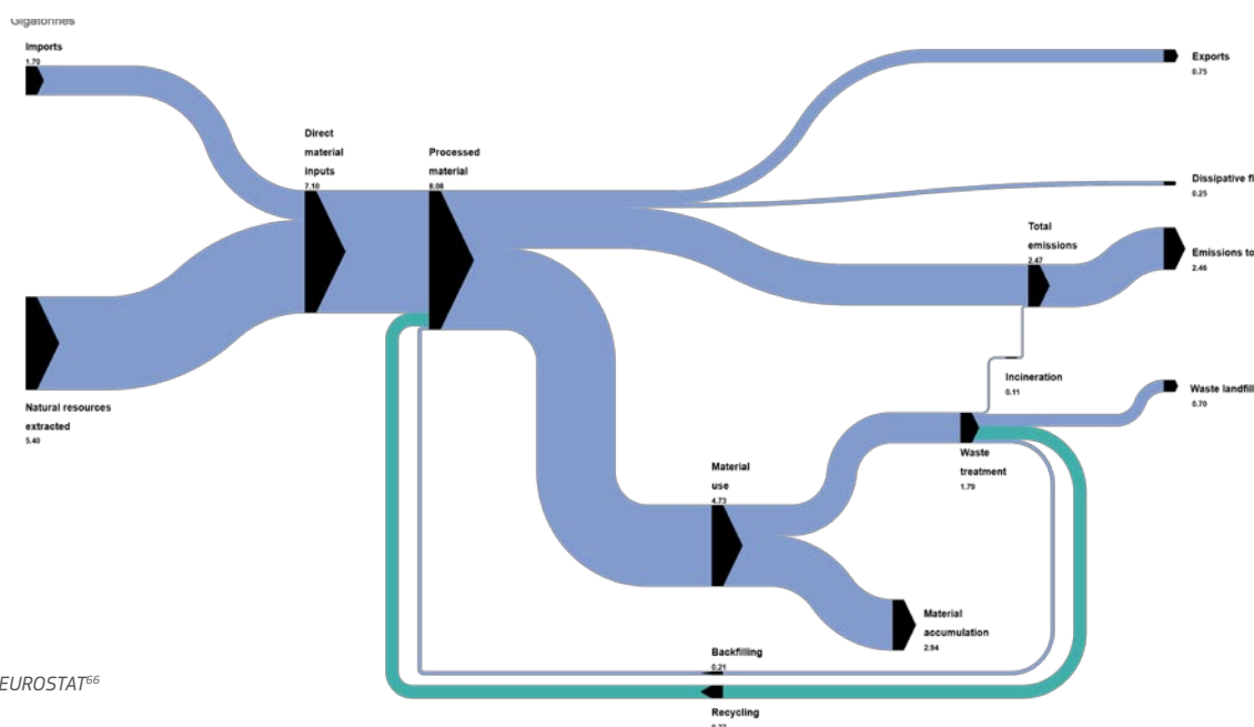
Figure 3.4 Material flow diagram for EU-27 (2018), Gt, true scale
