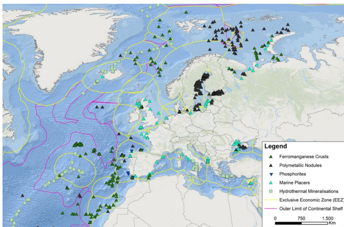
Figure 5.26 Marine mineral occurrences in EU waters
