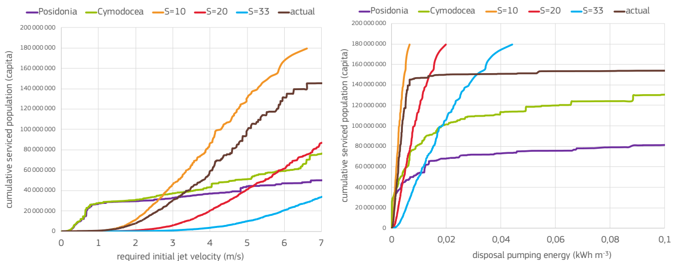
Figure 5.25 cumulative distribution of population serviced with increasing velocity and disposal energy for different dilution requirements
