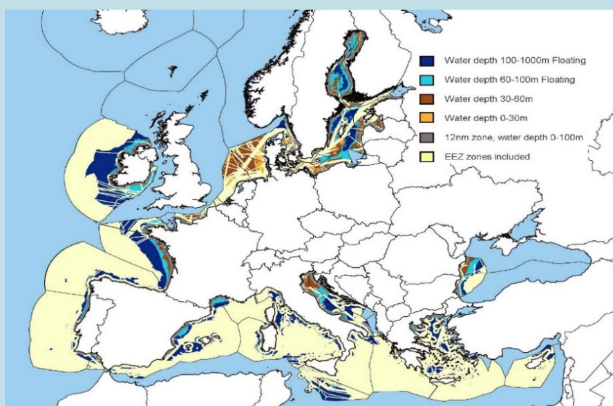
Figure 4.15 JRC ENSPRESO technical potentials for offshore wind in sea basins accessible to EU-27 countries.
