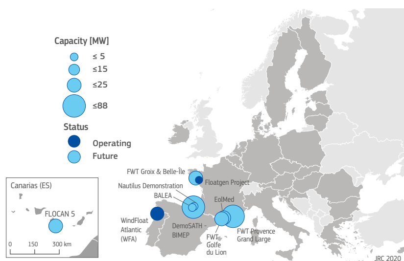
Figure 5.2 Location of EU and European floating offshore wind farms and large demonstrators (≥1MW) (announced and operational, as of December 2019).
