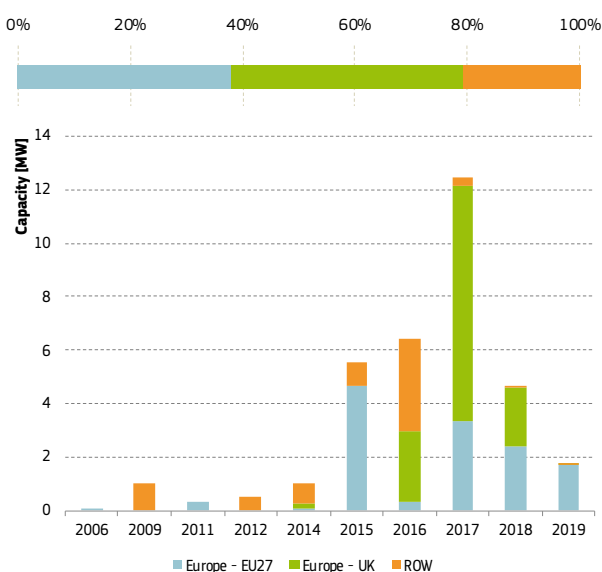
Figure 5.4 Global installed capacity post-BREXIT (excluding tidal range).
