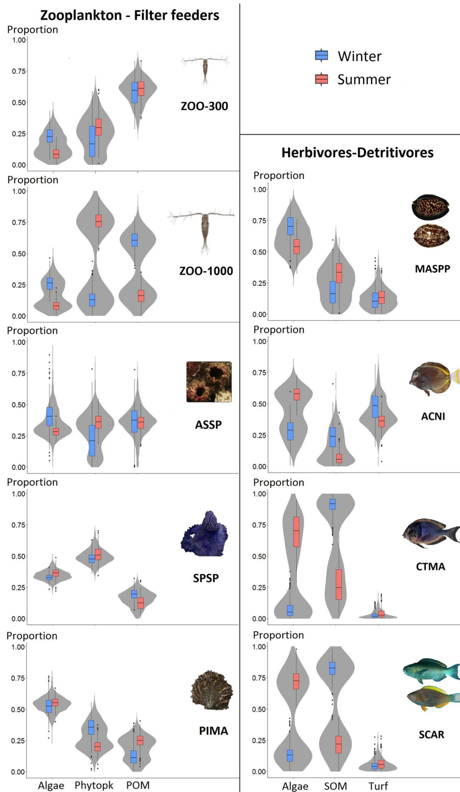
Figure 2. Relative proportions of the different OM sources for filter-feeders and zooplankton (left panel) and for herbivore-detritivores (right panel), based on SIAR mixing model outputs. Phytopk: Phytoplankton; POM: particulate organic matter; SOM: sedimentary organic matter. Violin plots represent the posterior distribution shape of the data (density estimation) in grey; boxplots represent median, interquartile ranges (red and blue boxes, depending on season), 95% credibility intervals (thin line) and outliers (black dots). ZOO-300: zooplankton 300–500 \mu\text{m} , ZOO-1000: zooplankton 1000–2000 \mu\text{m} , ASSP: ascidians, SPSP: Spheciospongia sp., PIMA: Pinctada margaritifera , ACNI: Acanthurus nigricans , CTMA: Ctenochaetus marginatus , SCAR: Scarinae ( Scarus koputea and S. rubroviolaceus ), MASPP: Mauritia spp.
