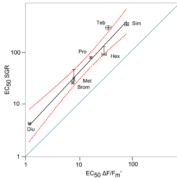
Figure 4. Linear relationship (black line) between inhibition of effective quantum yield ( \Delta F/F_m' ) and inhibition of specific growth rate (SGR) in Cladocopium goreauui by PSII herbicides (dashed red lines 95% confidence bands). Error bars are 95% CI for each \text{EC}_{50} value. Blue line indicates 1:1 relationship. Diu - diuron, Brom - bromacil, Hex - hexazinone, Met - metribuzin, Pro - propazine, Sim - simazine, Teb - tebuthiuron.
