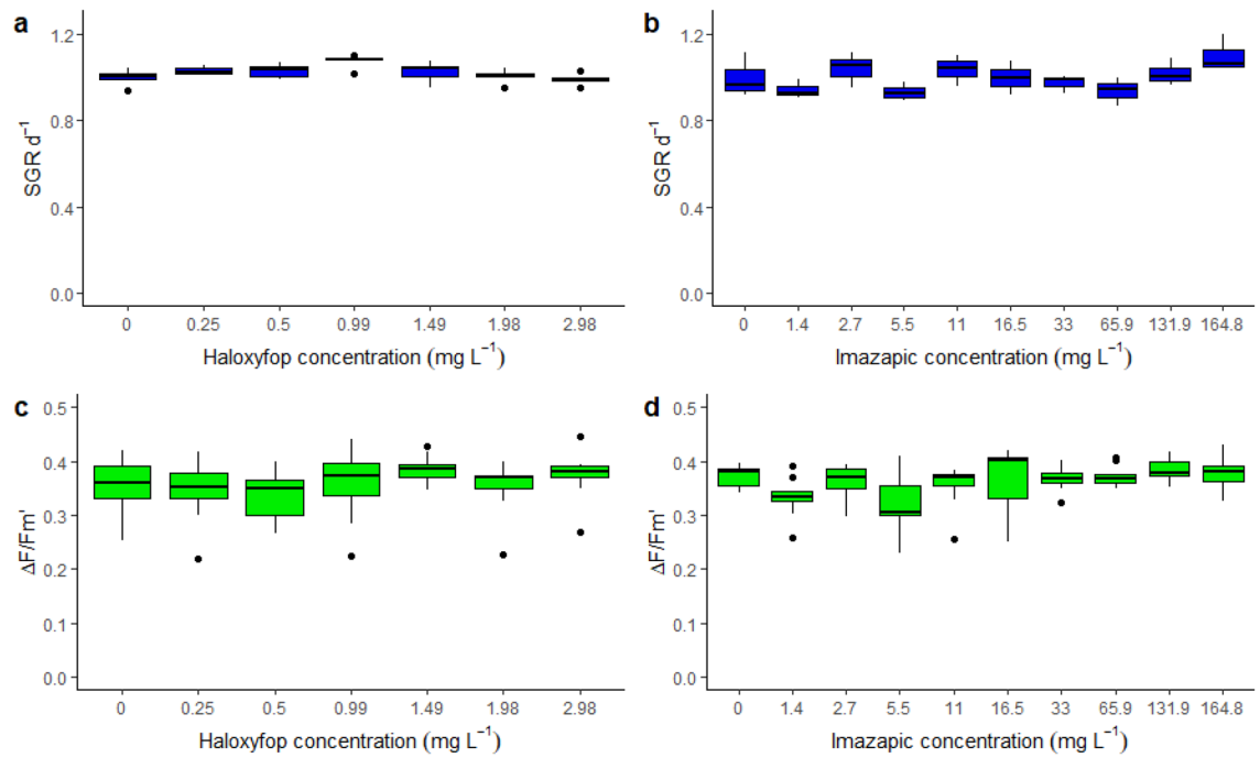
Figure 3. Response of Cladocopium goreauui to alternative non-PSII herbicides, haloxyfop and imazapic. Boxplots of the specific growth rate (SGR \text{day}^{-1} ) and effective quantum yields ( \Delta F/F_m' ) in response to haloxyfop (a,c) and imazapic (b,d). Note: all concentrations here are in \text{mg L}^{-1} .
