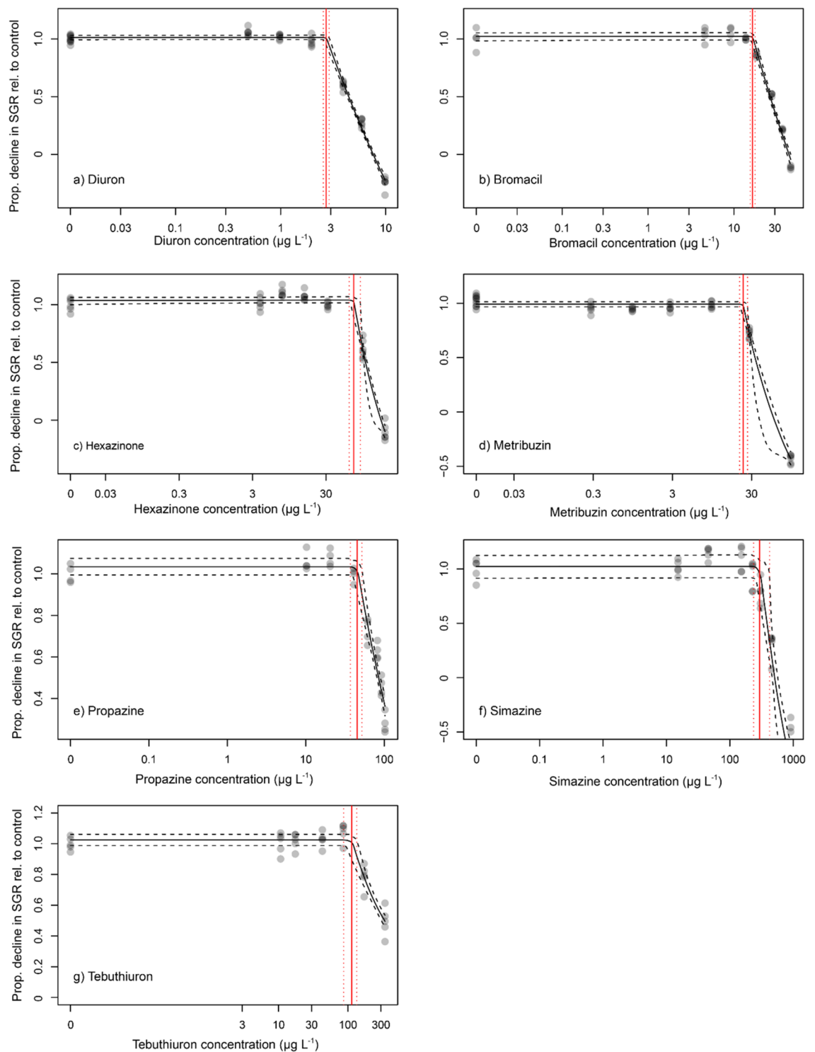
Figure 2. Proportional decline of specific growth rate (SGR) for Cladocopium goreauii relative to control treatment (solid black line) and 95% confidence intervals (black dashed line) to derive no effect concentration (NEC) (red line) and 95% confidence interval (red dashed line) of (a) diuron; (b) bromacil; (c) hexazinone; (d) metribuzin; (e) propazine; (f) simazine; and (g) tebuthiuron from Bayesian non-linear gaussian model fits. All concentrations in \mu\text{g L}^{-1} ( n = 4\text{--}6 per test).
