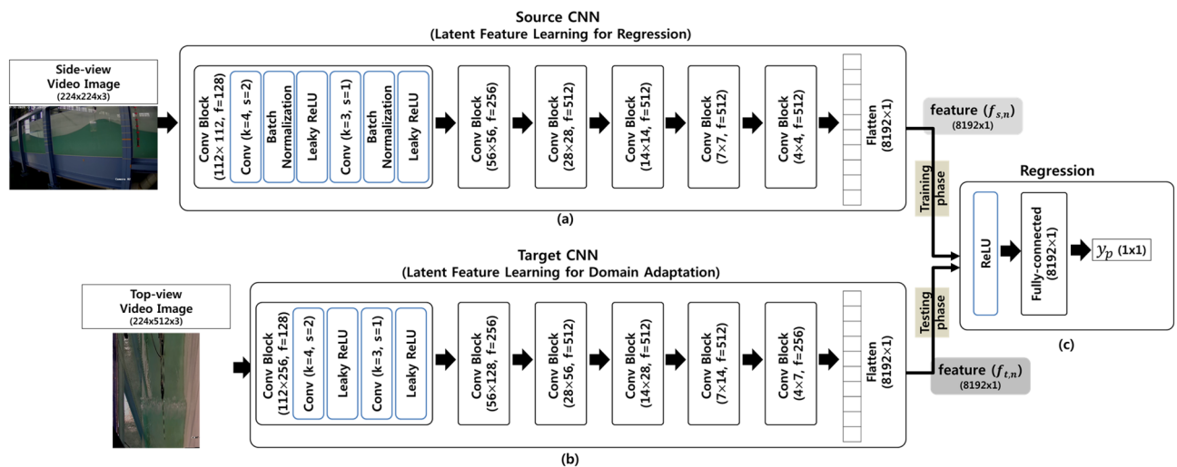
Figure 9. Architecture of (a) Source CNN , (b) Target CNN , and (c) Regression Network for water level estimation through domain adaptation.
