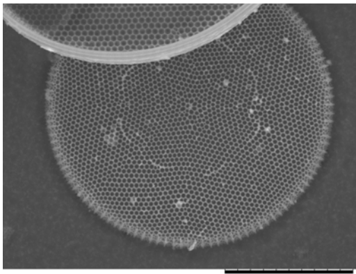
Thalassiosira anguste-lineate Synonym: Coscinodiscus angustelineatus (SEM, outer valve view, x2.0k, 30 µm scale)
