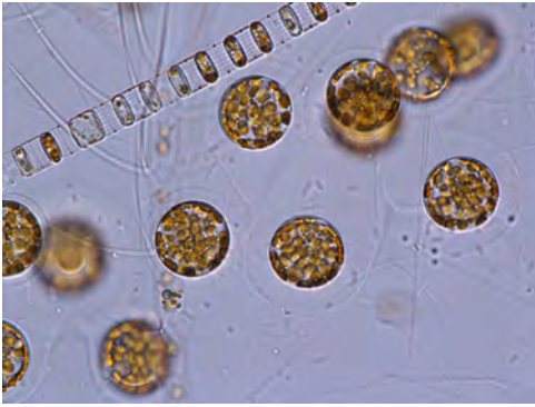
Thalassiosira subtilis (LM, valve view)
