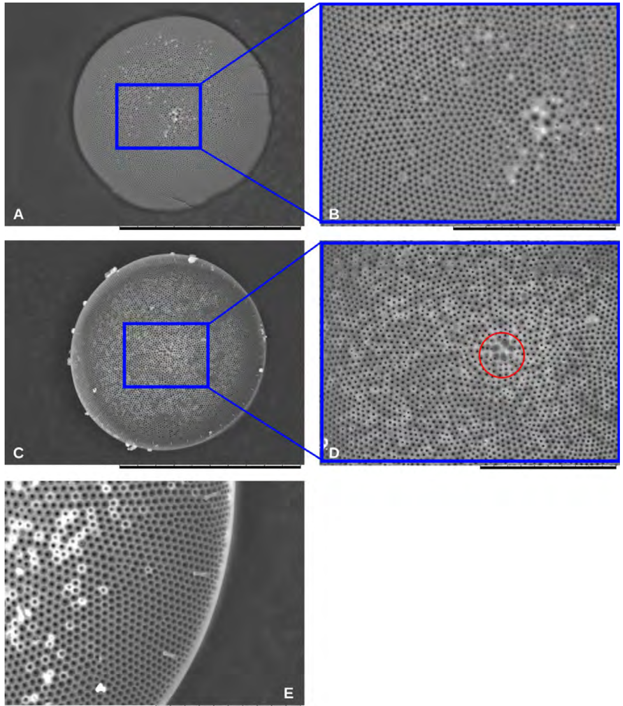
Figure 8. SEM images of Coscinodiscus oculus-iridis . (A) external valve face (x1.0k, 100 μm scale). (B) higher magnification of A shows “flower configuration” of pores only visible in external valve view (x3.0k, 30 μm scale). (C) internal valve face shows radial areolae and small circular pores (x1.0k, 100 μm scale). (D) higher magnification view of C shows central rosette (circled) (x2.5k, 30 μm scale). (E) marginal tube-like processes (range from ~7-10 μm apart) only visible in internal valve view (x4.0k, 20 μm scale).
