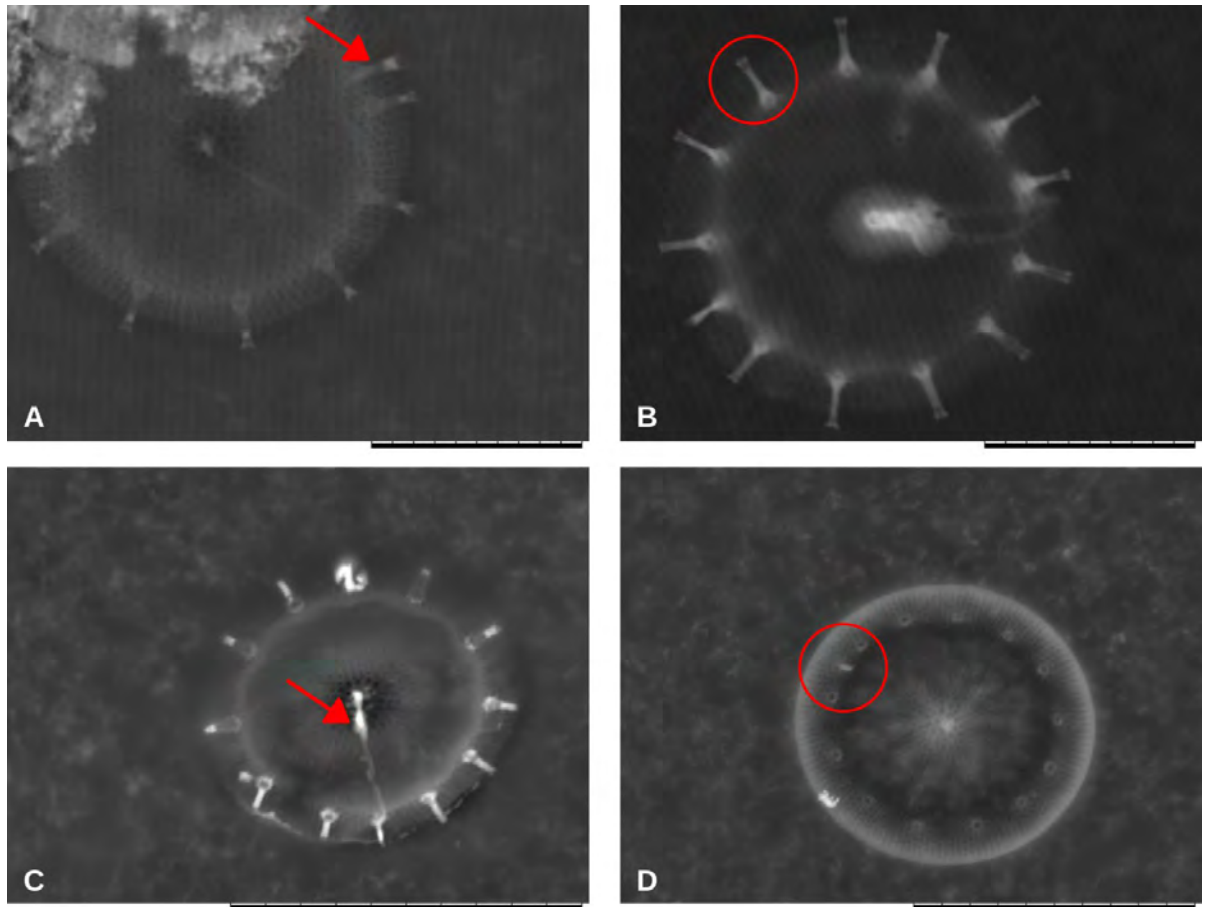
Figure 10. SEM images of Thalassiosira nordenskiöldii . (A) external valve face shows labiate process (arrow) and beveled edge (x6.0k, 10 µm scale). (B) external valve face shows strutted processes (circled) (x6.0k, 10 µm scale). (C) external valve face shows central process with filamentous structure attached (arrow) (x5.0k, 20 µm scale). (D) internal valve face shows linear, uniform areolae and labiate process (circled) (x4.0k, 20 µm scale).
