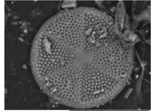
Actinoptychus senarius Synonym: Actinoptychus undulatus (SEM, outer valve view, x1.8k, 50 μm scale)
