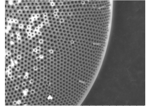
Thalassiosira oculus-iridis Synonym: Coscinodiscus oculus-iridis (SEM, inner valve view, x4.0k, 20 µm scale, image by author)
