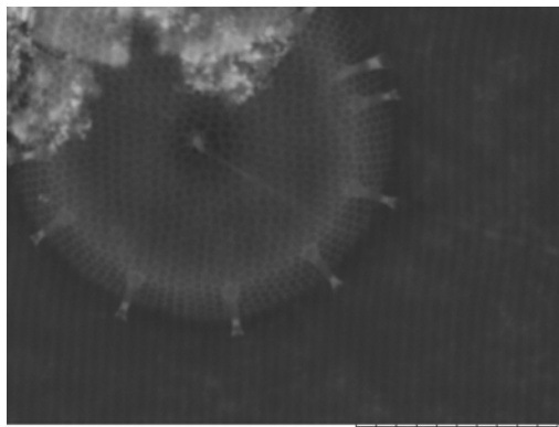
Thalassiosira nordenskiöldii (SEM, outer valve view, x6.0k, 10 µm scale, image by author)
