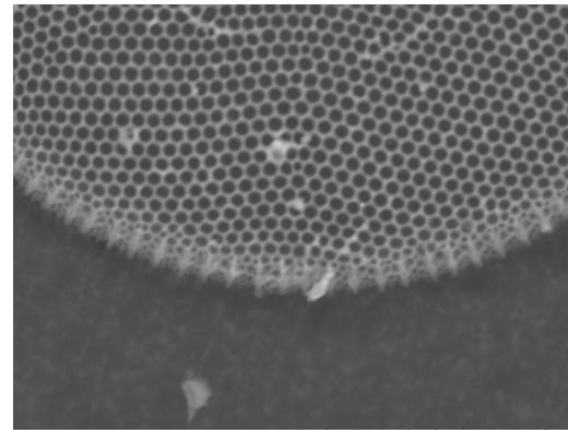
Thalassiosira anguste-lineate Synonym: Coscinodiscus angustelineatus (SEM, outer valve view, x4.0k, 20 µm scale)
