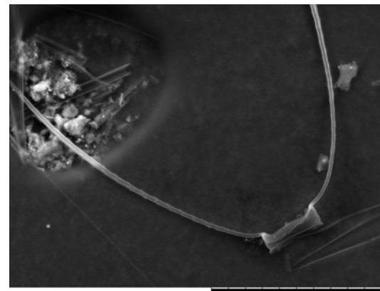
Chaetoceros sp. (SEM, girdle view, x1.5k, 50 \mu m scale)
