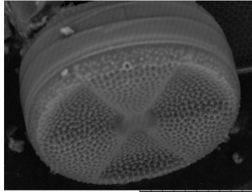
Actinoptychus senarius Synonym: Actinoptychus undulatus (SEM, x2.5k, 30 μm scale)
