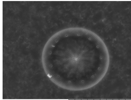
Thalassiosira nordenskiöldii (SEM, inner valve view, x4.0k, 20 µm scale, image by author)
