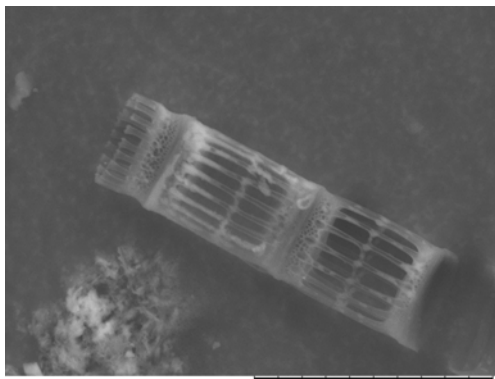
Skeletonema sp. (SEM, girdle view, x4.0k, 20 µm scale)
