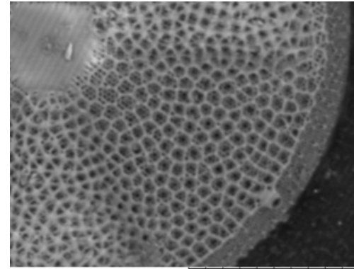
Actinoptychus senarius Synonym: Actinoptychus undulatus (SEM, outer valve view, x4.0k, 20 μm scale, image by author)
