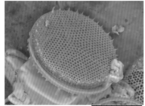
Thalassiosira lentiginosa Synonym: Coscinodiscus lentiginosus (SEM, x2.0k, 30 µm scale, image by author)
