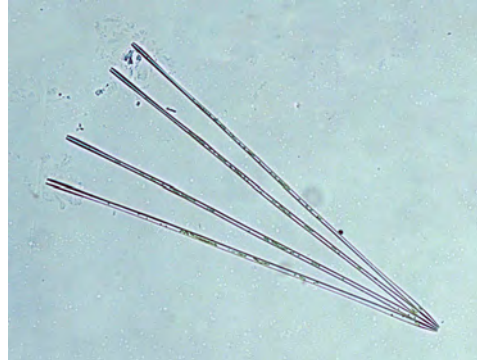
Lioloma pacificum Synonym: Thalassiothrix mediterranea var. pacifica (LM)
