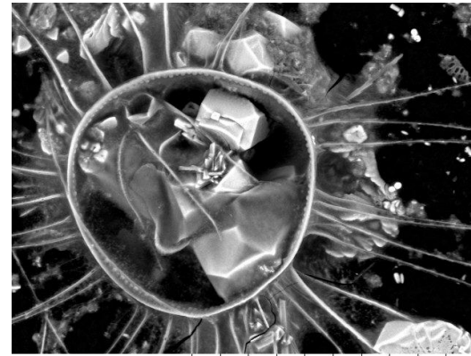
Corethron sp. (SEM, inner valve view, x1.0k, 100 µm scale)
