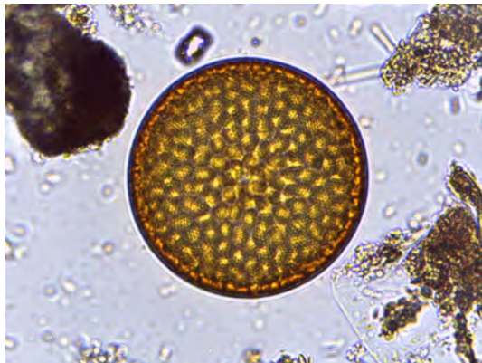
Coscinodiscus sp. (LM, valve view)
