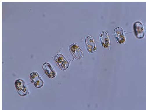
Thalassiosira nordenskiöldii (LM, girdle view)
