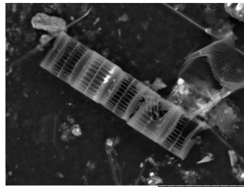
Skeletonema sp. (SEM, girdle view, x2.0k, 30 µm scale)
