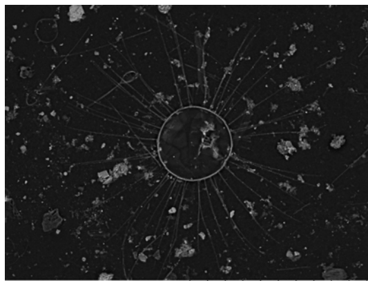
Corethron sp. (SEM, inner valve view, x400, 200 µm scale)
