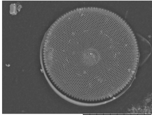
Thalassiosira anguste-lineate Synonym: Coscinodiscus angustelineatus (SEM, outer valve view, x1.5k, 50 µm scale)
