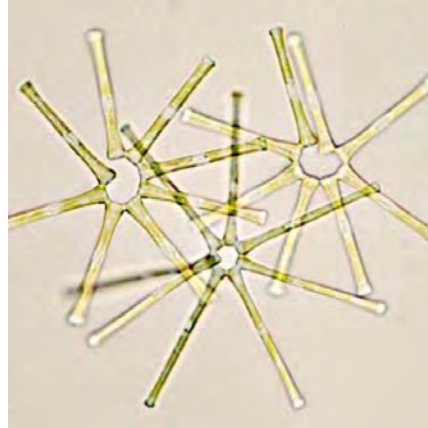
Asterionella japonica Synonym: Asterionellopsis glacialis (LM)
