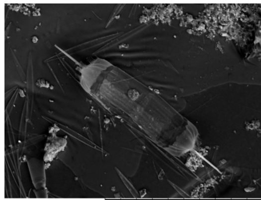
Ditylum sp. (SEM, girdle view, x500, 200 \mu m scale)
