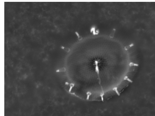
Thalassiosira nordenskiöldii (SEM, outer valve view, x5.0k, 20 µm scale, image by author)
