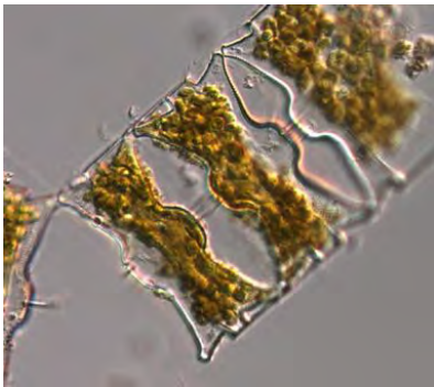
Odontella aurita Synonym: Biddulphia aurita (LM, girdle view, image by A-T. Skjevik)
