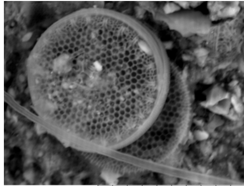
Chaetoceros decipiens (SEM, valve view, x5.0k, 20 µm scale)
