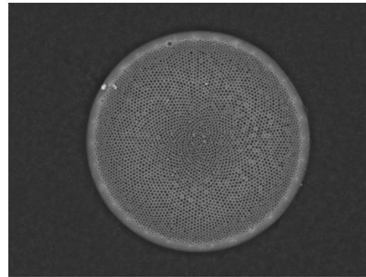
Coscinodiscus curvatulus Synonym: Actinocyclus curvatulus (SEM, outer valve view, x1.2k, 50 µm scale, image by author)
