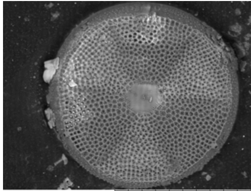
Actinoptychus senarius Synonym: Actinoptychus undulatus (SEM, outer valve view, x1.8k, 50 μm scale, image by author)
