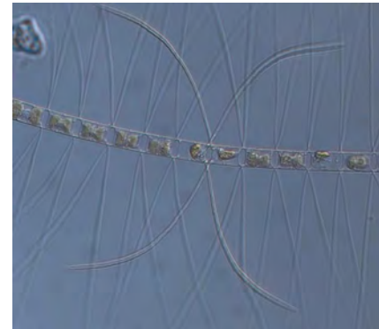
Chaetoceros affinis (LM, girdle view, image by A-T Skjevik)
