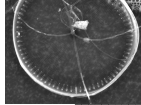
Thalassiosira rotula Synonym: Coscinodiscus rotulus (SEM, inner valve view, x4.0k, 20 µm scale)
