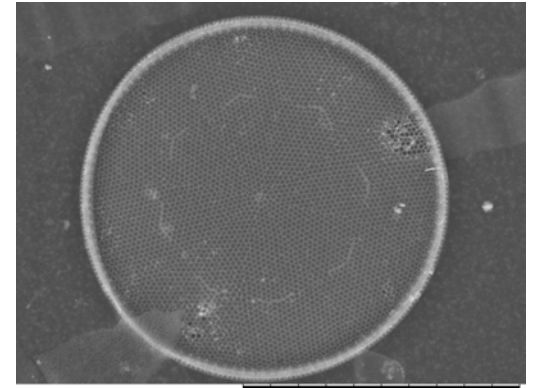
Thalassiosira anguste-lineate Synonym: Coscinodiscus angustelineatus (SEM, inner valve view, x1.8k, 50 µm scale)
