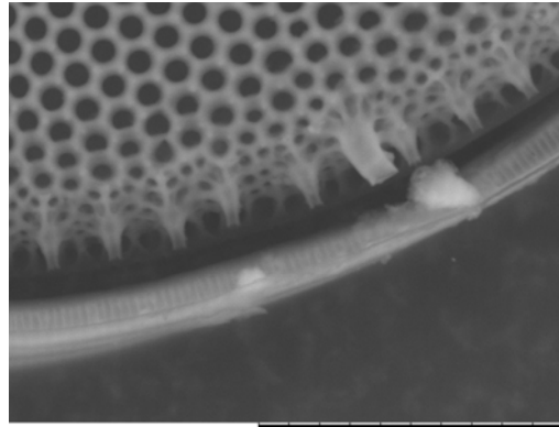
Thalassiosira anguste-lineate Synonym: Coscinodiscus angustelineatus (SEM, outer valve view, x9.0k, 10 µm scale)
