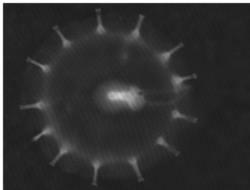
Thalassiosira nordenskiöldii (SEM, outer valve view, x6.0k, 10 µm scale, image by author)
