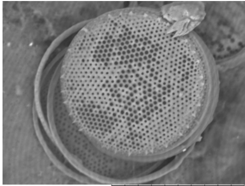
Thalassiosira lentiginosa Synonym: Coscinodiscus lentiginosus (SEM, x1.8k, 50 µm scale, image by author)
