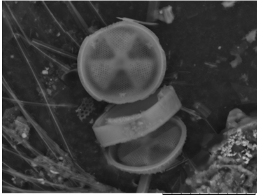
Actinoptychus senarius Synonym: Actinoptychus undulatus (SEM, x2.0k, 30 μm scale)
