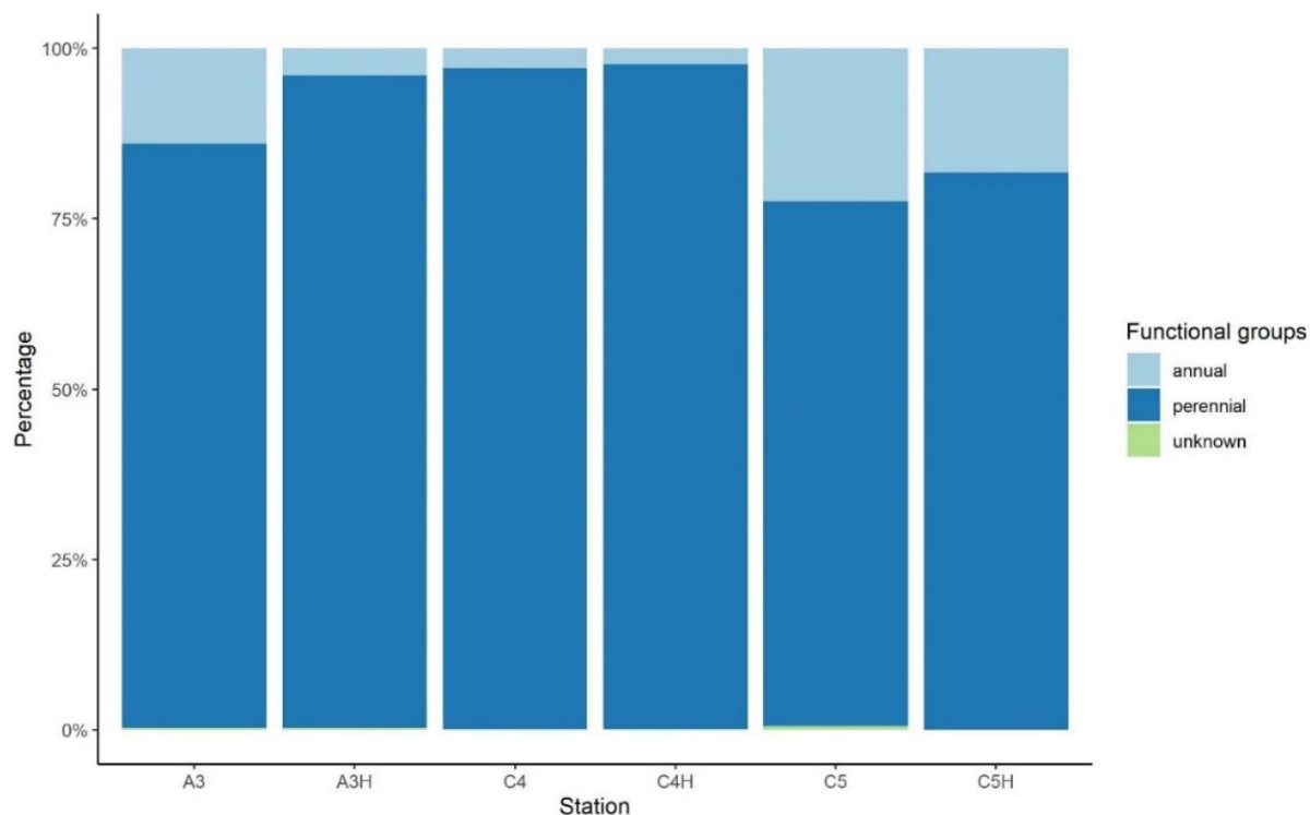
Figure 18 – Stacked bar plot comparing percentage coverage of annual and perennial algal species at each station sampled spring and summer. A in the station name indicates aquaculture station and C control station. A3 and A3H is the same station, but the H in the station name indicates that the data was collected in summer while name without H was sampled in spring.
