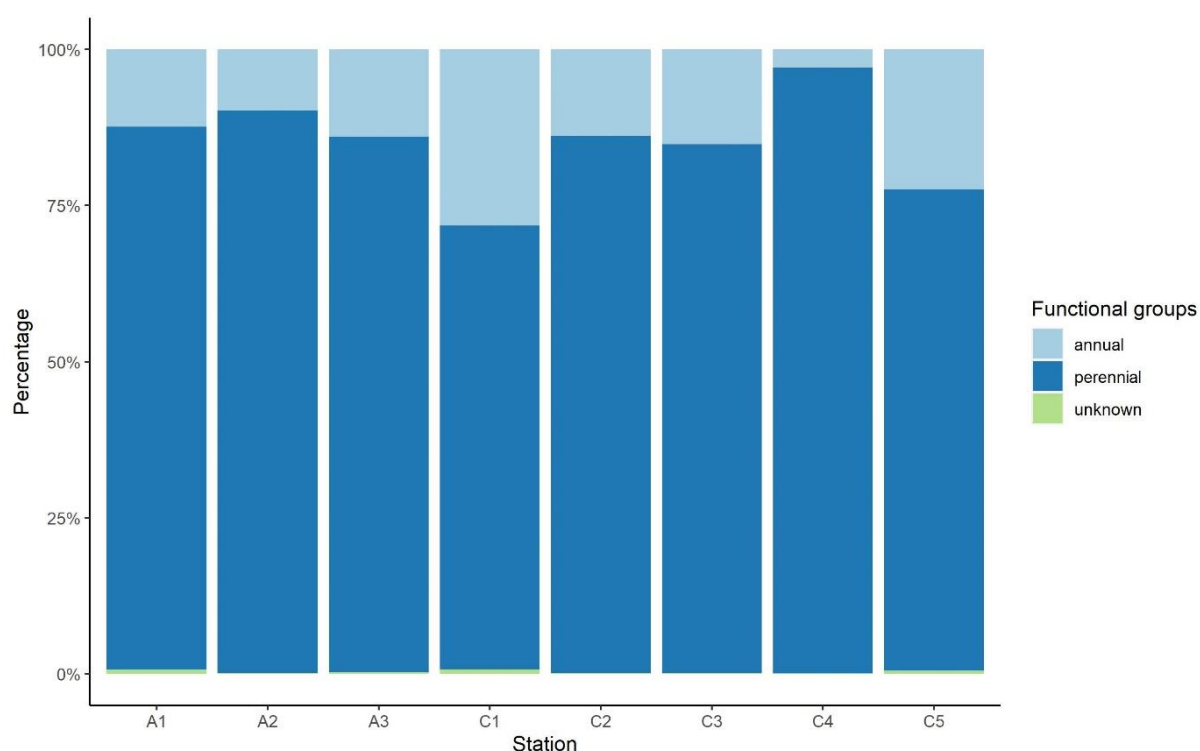
Figure 11 – Proportion of annual and perennial algae coverage at each station. A1-3 implies aquaculture station 1-3 and C1-5 implies control station 1-5.
