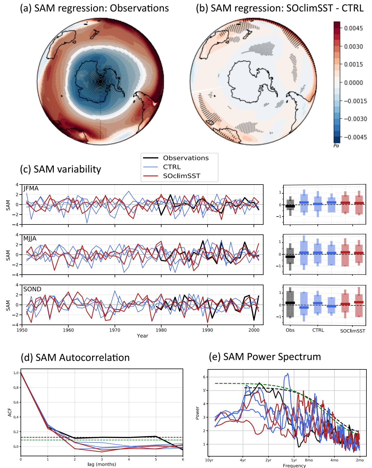
Figure 2. (a) Regression of monthly MSLP anomalies onto SAM in ERA5 reanalyses (1979–2001), and (b) difference between the regression of monthly MSLP anomalies onto SAM in SOclimSST runs and the regression of monthly MSLP anomalies onto SAM in CTRL runs (1951–2001). As in Fig. 1, stippling indicates robustness in the sign of the ensemble-mean difference, where the sign of all six individual differences (each SOclimSST run minus each CTRL run) is the same. (c) SAM timeseries for observations and each simulation for JFMA, MJJA and SOND, with corresponding bar plots on the right showing the median, 25th and 75th percentiles and \pm one standard deviation for each timeseries. (d) Autocorrelation, and (e) power spectrum density in SAM across observations, CTRL and SOclimSST, with dashed lines showing the 95% confidence level for observations (black) and model runs (green). SAM has been calculated based on the Gong and Wang (1999) definition 35 and all monthly data has been linearly detrended prior to analysis. Figure produced using Python ( https://docs.python.org/3.0/ ).
