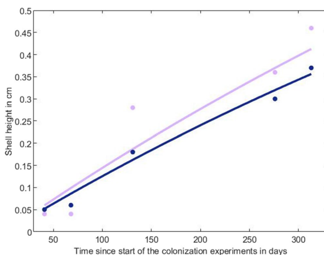
Figure 1. Observed (dots) and predicted (lines) data on the growth of Xylonorora atlantica in shell height before and after using the abj-DEB model. Data from the pine substrate are in purple, and those from the oak substrate are in blue. The observed data were obtained from in situ colonization experiments at a depth of 100 m 22 and were the mean values of 8 to 174 individuals depending on the sampling period or wood type. The relative error of the data predicted (RE) for the pine substrate (purple) was 0.19, and the RE for the oak substrate (blue) was 0.08.
