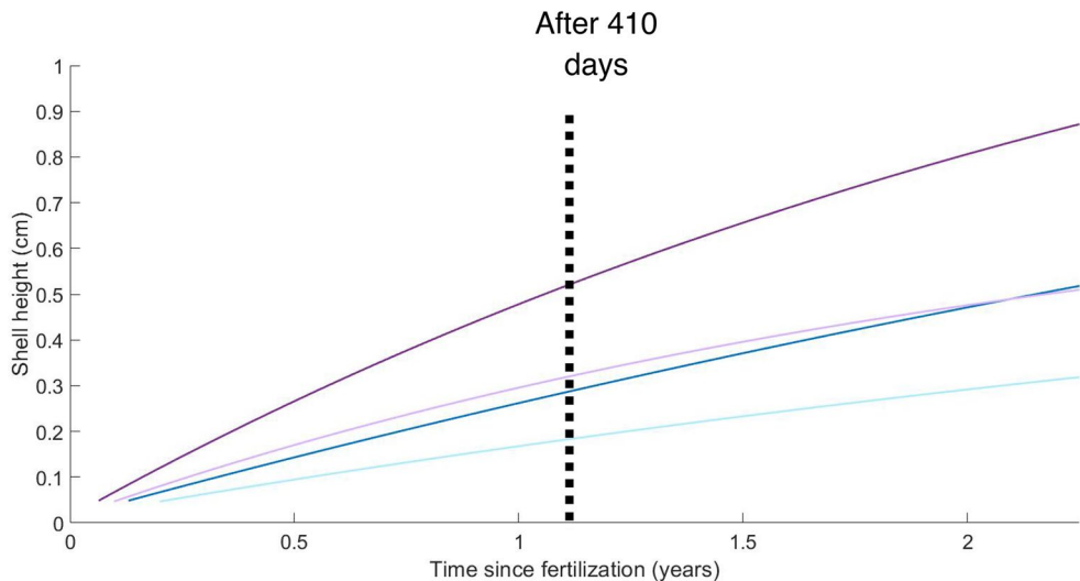
Figure 3. Prediction of the abj-DEB model of the evolution of the shell height of Xylonor atlantica under different environmental scenarios. At 2300 m in depth ( T = 4\text{ }^{\circ}\text{C} ) with food level f = 0.5 (light blue) and f = 1 (dark blue); at 100 m in depth ( T = 11\text{ }^{\circ}\text{C} ) with f = 0.5 (light purple) and f = 1 (dark purple) up to the lifespan at 4\text{ }^{\circ}\text{C} (821 days).
