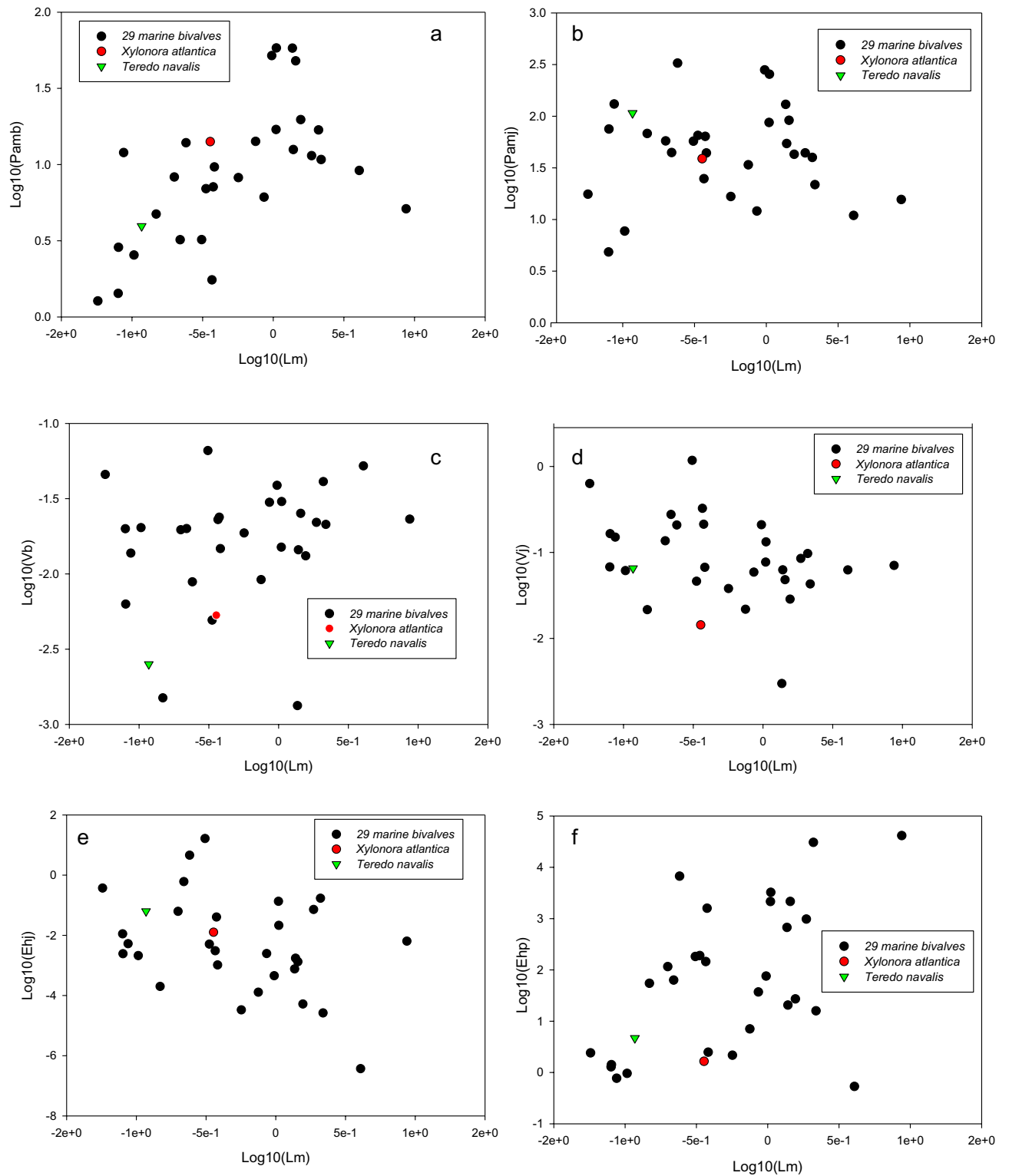
Figure 2. Interspecific comparison of abj-DEB parameter values of 29 marine bivalves with those of the deep-sea wood borer Xylonor atlantica and the shallow wood borer Teredo navalis , scaled to body size (Lm: maximum structural length) (a) Pamb, maximum assimilation rate at birth \{\dot{p}_{Am}\}_b , (b) Pamj, maximum assimilation rate after metamorphosis \{\dot{p}_{Am}\}_j ; (c) Vb, energy conductance at birth \dot{v}_b ; (d) Vj, energy conductance after metamorphosis \dot{v}_j ; (e) Ehj, energy threshold after metamorphosis E_{Hj}^p , and (f) Ehp, energy threshold at puberty E_{Hp}^p . The black circles are the values for the 29 marine bivalves for which an abj-DEB model was applied. The red circles are the DEB parameter values of X. atlantica . The green triangles are the DEB parameter values of T. navalis .
