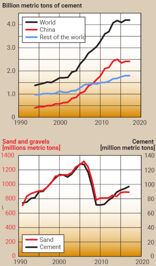
Figure 1: There are no global monitoring on the use of sand. However, cement is well reported. Tracking this data shows that the production of cement has tripled in the last two decades.
