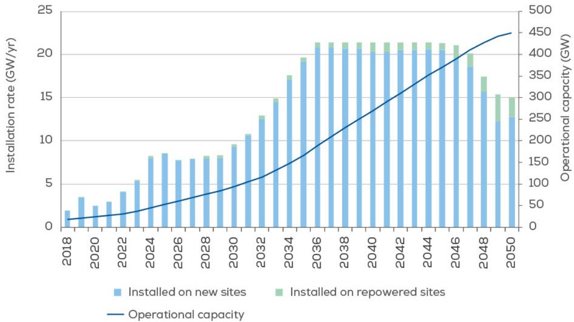
Installation rate required to achieve 450 GW by 2050
