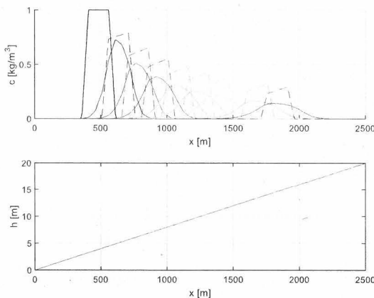
Figure 2 – Upper figure: temporal variation of suspended sediment concentration calculated using the updated ERIA scheme (solid lines) and comparison with the analytical solution (dashed lines). Lower figure: increase of the water depth along the channel.
