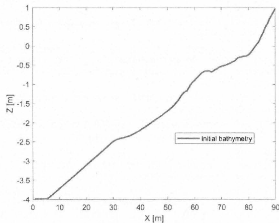
Figure 5 – Initial bathymetry for the CROSSTEX experiments under investigation [20].
