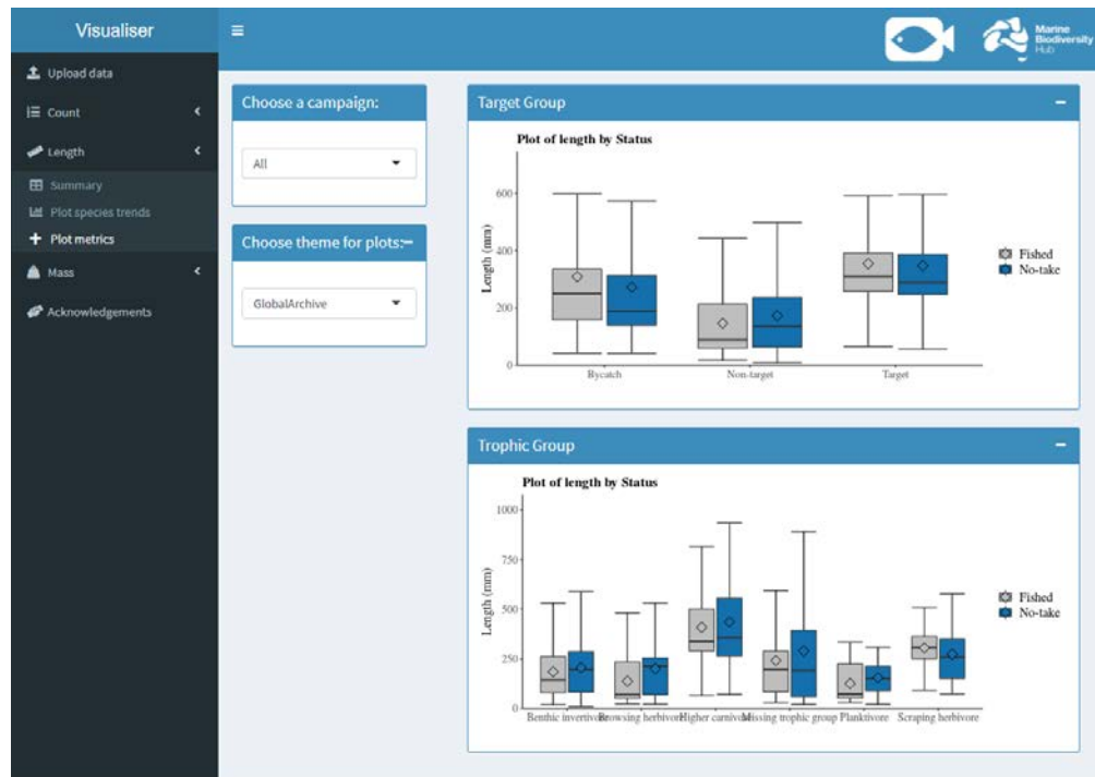
Figure 13 Length metrics
