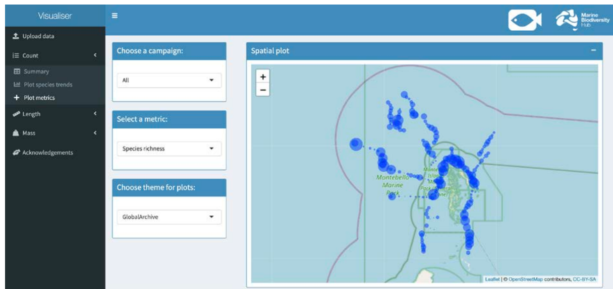
Figure 10 Count metrics
