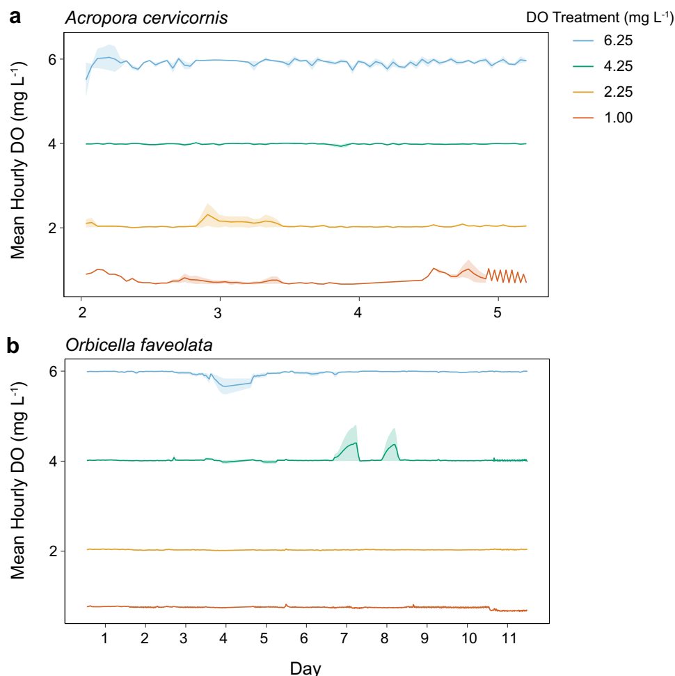
Figure 1. Dissolved oxygen treatment conditions. Mean hourly dissolved oxygen (DO) concentrations in treatment tanks ( n=3 ), with SD shown as shaded areas around the mean. Oxygen treatments were maintained through an oxygen-feedback, with continuous monitoring every 15 s for the duration of each experiment. (a) Acropora cervicornis was exposed to treatment conditions for 5 days and (b) Orbicella faveolata for 11 days. Day 1 represents the start of the experiment and first day of biological measurements.
