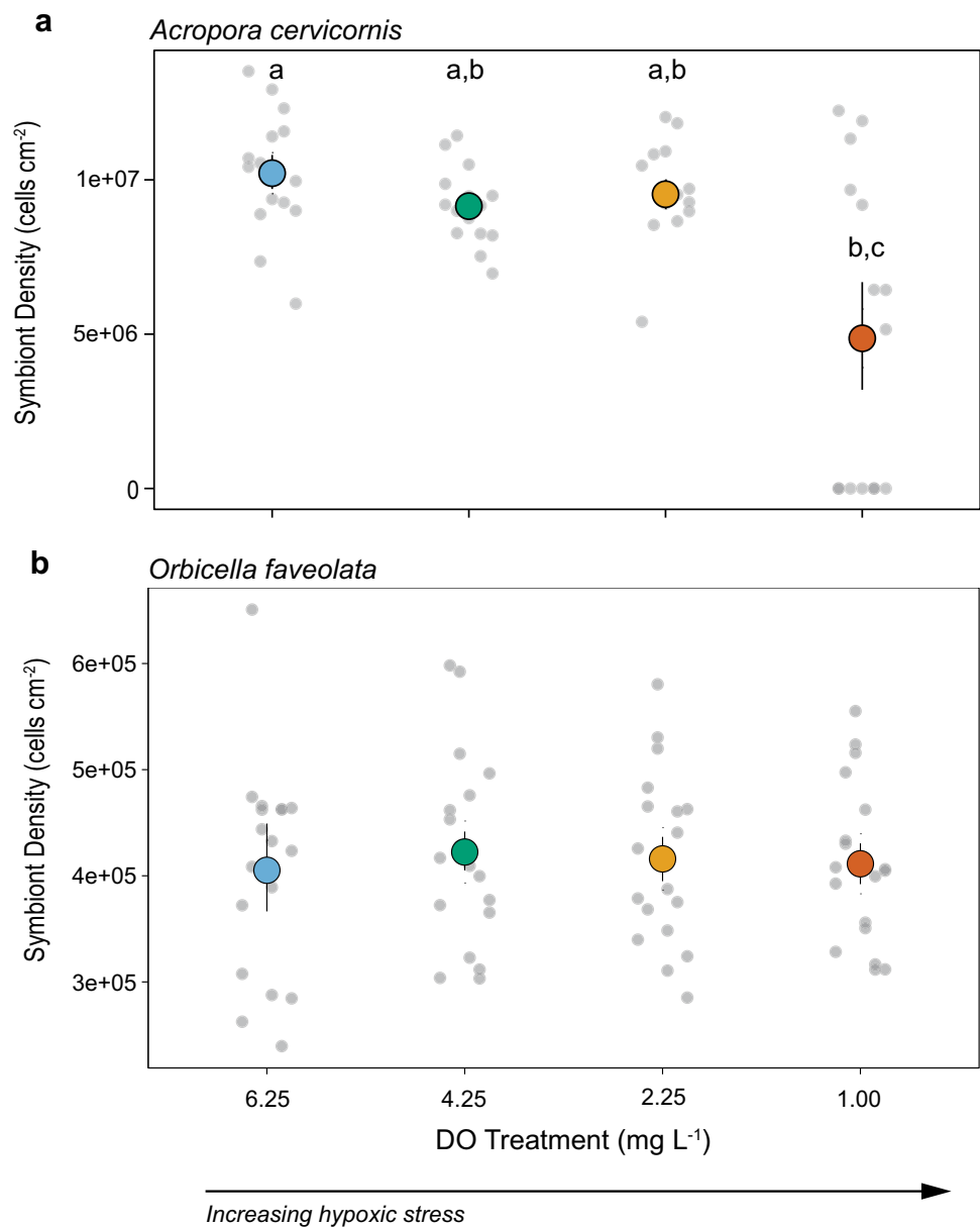
Figure 4. Coral symbiont densities under deoxygenation. (a) Mean ± SE symbiont densities at the end of the 5-day experiment for Acropora cervicornis and (b) the 11-day experiment for Orbicella faveolata (n = 3). The grey circles show individual data points and colored circles represent means across all genotypes within a treatment. Treatments with different lower-case letters are statistically different at P < 0.05 .
