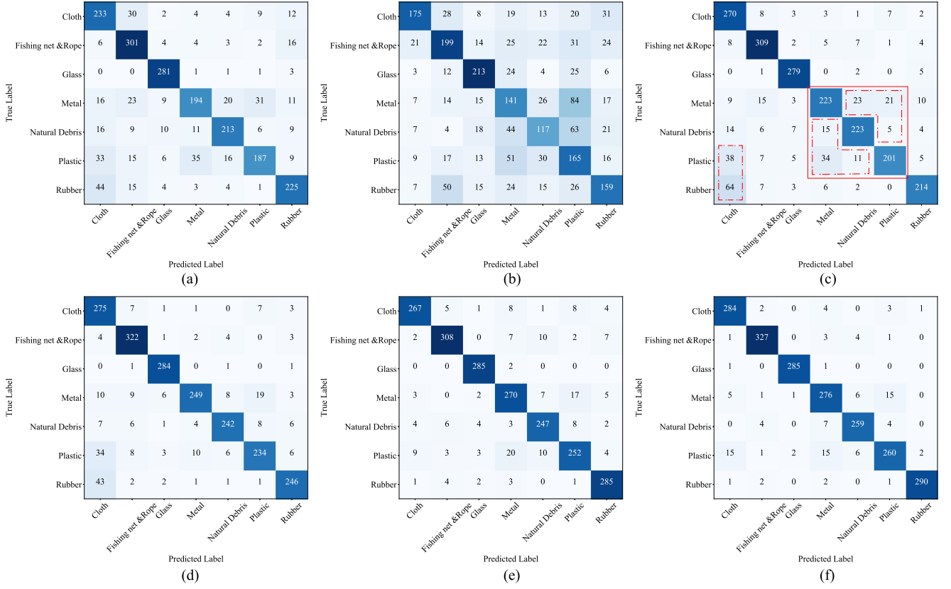
Fig. 11. Confusion matrix of each model on the DDI dataset.
