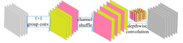
Fig. 4. Main unit/module used by Shuffle-Xception network (SX unit/module).
