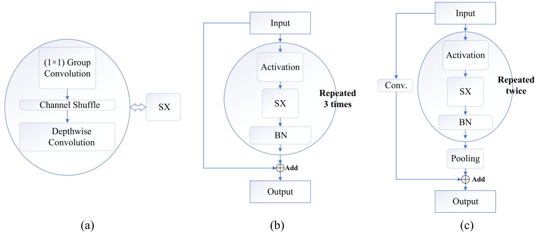
Fig. 5. SX modules combined with the residual connection. (a) gives the SX module. (b) and (c) are the two main modules of the Shuffle-Xception network. “Activation-SX-BN” is repeated three times in module (b), but twice in module (c).
