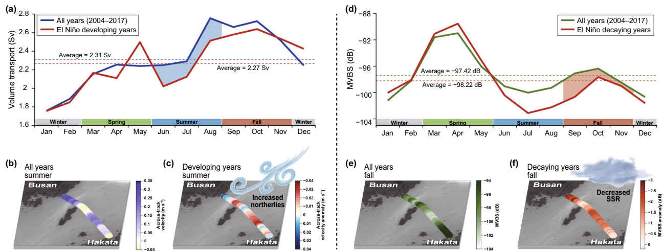
Figure 4. Climatic impact of El Niño on volume transport and the mean volume backscattering strength (MVBS) across the Korea/Tsushima Strait. (a) Monthly average of volume transport during all years and El Niño developing years (2009 and 2015). The shaded area indicates the difference in summer (JJA) volume transport between the two time windows. (b) Averaged summer across-track velocities during all years. (c) Averaged summer across-track velocity anomalies during El Niño developing years. (d) Monthly average MVBS during all years and El Niño decaying years (2010 and 2016). The shaded area indicates the difference in fall (SON) MVBS between the two time windows. (e) Averaged fall MVBS during all years and (f) Averaged fall MVBS anomalies during El Niño decaying years. The figure was created using MATLAB (ver. 9.9.0.1592791 (R2020b) Update 5). The bathymetry is based on the SRTM30_PLUS dataset ( https://topex.ucsd.edu/ ).
