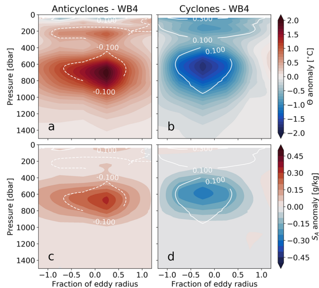
Figure 4. Mesoscale eddy properties at the RAPID/MOCHA mooring WB4. (a) Mean \Theta anomaly of anticyclonic eddies that pass RAPID/MOCHA mooring WB4. Mooring observations of \Theta anomaly are binned according to the distance (normalised with respect to the eddy radius) of the eddy from the mooring. The value at a given eddy radius fraction is therefore the mean of all eddies that passed within that fraction of the eddy radius. White contours show \rho anomaly (units \text{kg m}^{-3} ). (b) As in (a) but for cyclonic eddies. (c) As in (a) but showing mean S_A anomaly. (d) As in (b) but showing mean S_A anomaly.
