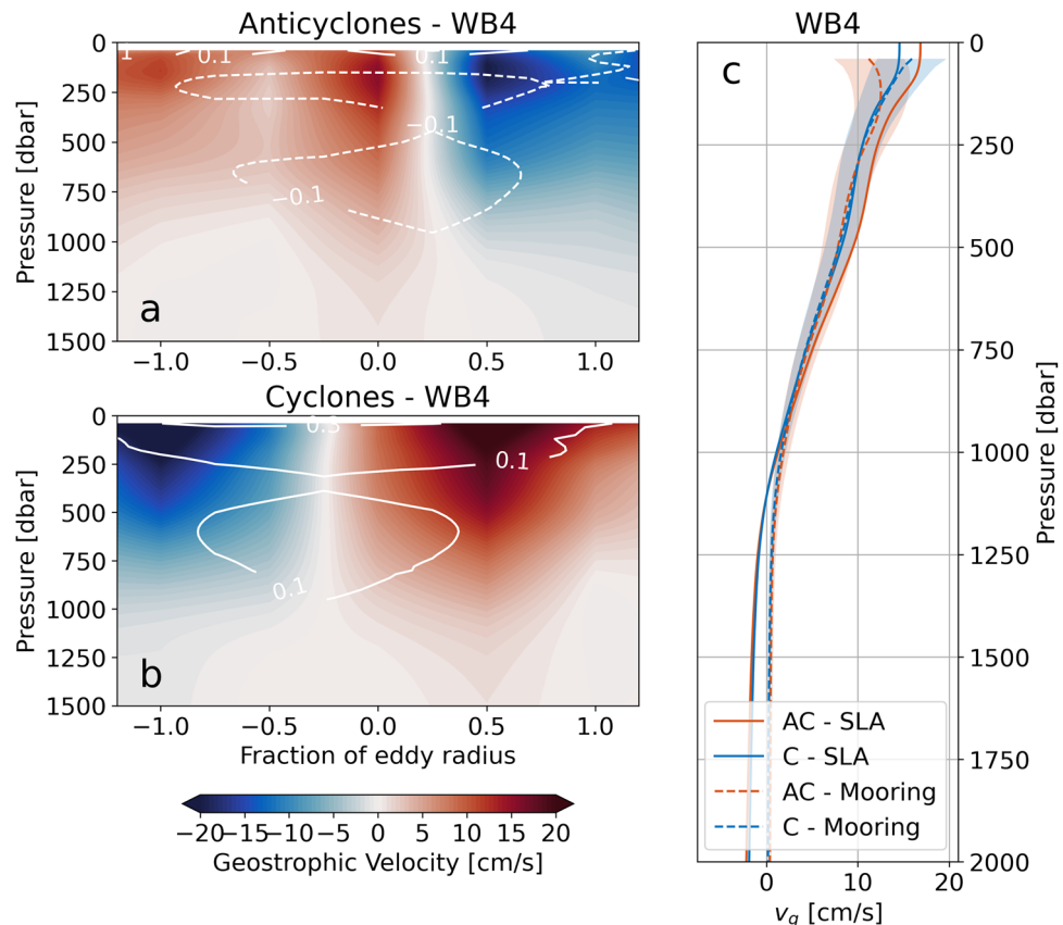
Figure 5. Mesoscale eddy geostrophic velocity at the RAPID/MOCHA mooring WB4. (a) Meridional geostrophic velocity calculated using the composite density ( \rho ) sections from the RAPID/MOCHA mooring WB4 for anticyclonic eddies. White contours show density anomaly ( \rho' ) units \text{kg m}^{-3} . (b) As in (a) but for cyclonic eddies. (c) A comparison between geostrophic velocity at the RAPID/MOCHA mooring WB4 (dashed lines) and the velocity profiles estimated from surface geostrophic velocity derived from altimetry data, assuming sub-surface first mode baroclinic structure (solid lines) for anticyclonic (orange) and cyclonic (blue) eddies. The shading indicates an uncertainty range for the mooring-based estimate using Monte-Carlo based bootstrapping to calculate upper and lower bounds for density.
