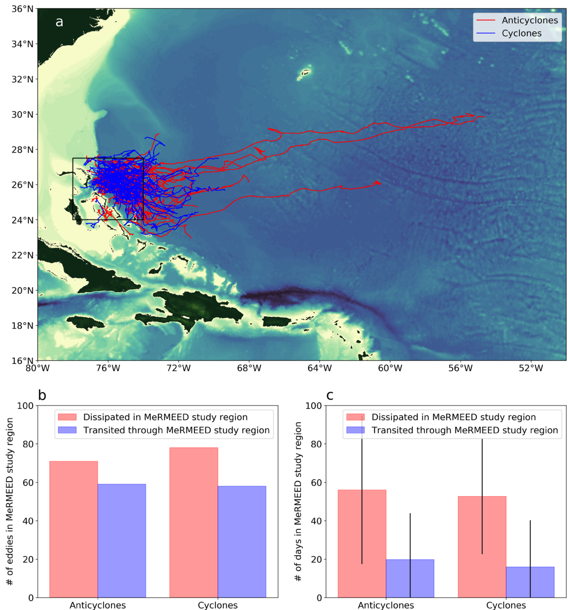
Figure 2. Eddy trajectories and statistics in the MeRMEED study region. (a) Trajectories of anticyclonic (red) and cyclonic (blue) eddies that enter the MeRMEED study region marked by the black box during their lifespan between 1993 and 2018. (b) The number of anticyclonic (left) and cyclonic (right) eddies that dissipate within the MeRMEED study region (red bar), and that transit through the MeRMEED study region (blue bar). (c) The average number of days spent in the MeRMEED study region for those anticyclonic (left) and cyclonic (right) eddies that either dissipate in the MeRMEED study (red bar) region or transit through the MeRMEED study region (blue bar). The vertical black lines represent the one standard deviation about the mean. The map in panel (a) was created using the Python packages cartopy v0.18 and matplotlib v3.3.4, and ETOPO1 bathymetry.
