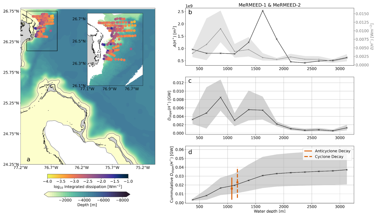
Figure 7. Turbulent dissipation in the MeRMEED study region. (a) Integrated turbulent dissipation measured using a tethered vertical microstructure profiler during the MeRMEED fieldwork campaign. Bathymetry from ETOPO-1 is shown in the main panel and swath-based bathymetry is shown in the inset panel that shows the MeRMEED cruise region. The grey contour is the 250 m depth contour. (b) Total isobath area ( A(H^*) ) for bins of water depth based on ETOPO-1 for the entire domain shown in (a) and integrated isobath dissipation rate ( \bar{\epsilon}(H^*) ) averaged in depth bins based on the depth at the location of the profile. (c) Turbulent dissipation rate ( D_{slope}(H^*) ) from the product of A(H^*) and \bar{\epsilon}(H^*) . (d) D_{slope}(H^*) accumulated in depth space shown with the eddy kinetic energy decay rate for anticyclones (orange solid line) cyclones (orange dashed line) between 10 and 60 days before eddy decay from Fig. 6c. The shading represents an estimate of the uncertainty in the mean isobath integrated dissipation rate calculated using Monte-Carlo based bootstrapping. The map in panel (a) was created using the Python packages cartopy v0.18 and matplotlib v3.3.4, with ETOPO1 bathymetry and GSHHG coastline data.
