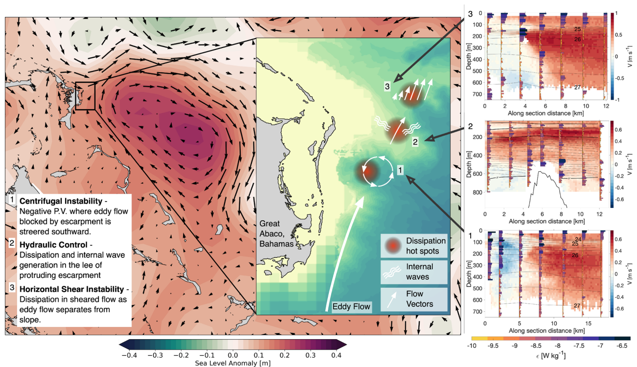
Figure 1. Eddy flow topography interactions. A schematic representation of the varied interactions between the flow of an anticyclonic eddy and the steep and rough slope offshore of Great Abaco, Bahamas. The large panel shows the sea level anomaly (SLA; contours) from October 31 2017 and associated surface geostrophic flow (black arrows). The positive SLA anomaly is an anticyclonic eddy impinging on the eastern slope of the Lucayan Archipelago. The inset panel shows the bathymetry (yellow–blue contours) for a region where the MeRMEED fieldwork took place, and highlights the key regions of eddy flow-topography interactions: (1) Generation of centrifugal instability; (2) Hydraulic control; (3) Generation of horizontal shear instability. The three right hand panels show vessel mounted acoustic Doppler current profiler-based meridional velocity ( V ) and density ( \rho ; black contours) in each of the three key regions. The stacked bar plots show vertical microstructure-based estimates of the turbulent dissipation in 10 m bins. Each are scaled by 10^{-10} \text{ W kg}^{-1} , and the colour represents the dissipation rate with a logarithmic scale. For more details see Evans et al. 16 . The maps were created using the Python packages cartopy v0.18 and matplotlib v3.3.4, using coastline data from the Global Self-consistent Hierarchical High-resolution Geography (GSHHG; v2.3.7 https://www.ngdc.noaa.gov/mgg/shorelines/ ) and a combination of ETOPO1 and multibeam-based bathymetry.
