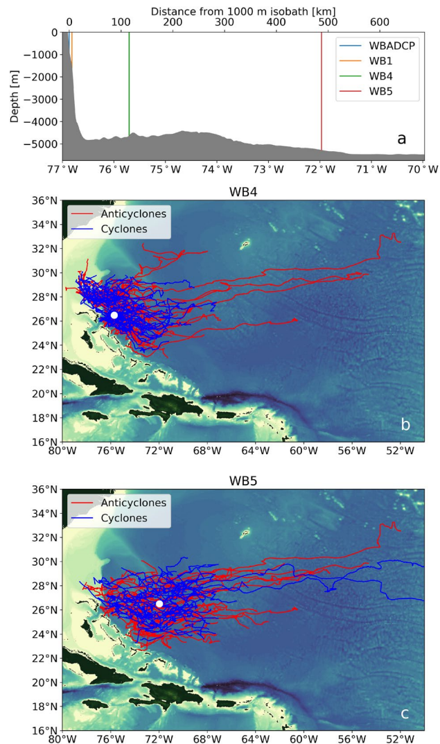
Figure 3. Mesoscale eddies at the RAPID/MOCHA moorings. (a) Location of the western boundary RAPID/MOCHA moorings offshore of the Bahamas. The gray shaded area shows the bathymetry. (b) Trajectories of anticyclonic (red) and cyclonic (blue) eddies that pass within two eddy radii of the RAPID/MOCHA mooring WB4 during the mooring deployment (2008–2018). (c) As in (b) but for the RAPID/MOCHA mooring WB5 during the mooring deployment (2004–2014). The maps in panel (b,c) were created using the Python packages cartopy v0.18 and matplotlib v3.3.4, and ETOPO1 bathymetry.
