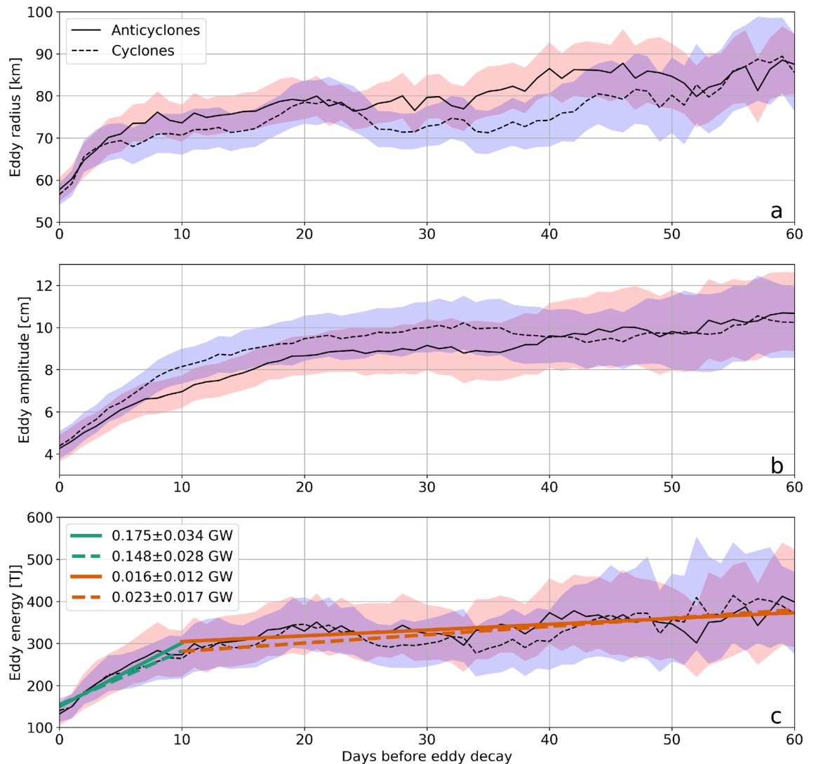
Figure 6. Mesoscale eddy decay rate. (a) Mean eddy radius of anticyclonic (red) and cyclonic (blue) eddies that dissipate within the MerMEED study region, shown as a function of days before decay. The shading represents an estimate of the uncertainty in the eddy radius calculated using Monte-Carlo based bootstrapping. (b) As in (a) but for eddy amplitude. (c) As in (a) but for eddy kinetic energy. The coloured lines are a linear fit to the eddy kinetic energy curves for the intervals 0–10 days before decay and 10–60 days before decay. The gradient of each coloured line is shown in the legend where the uncertainty range is estimated from the mean difference between the gradient of the upper and lower bounds (represented by the shading) and the central curve.
