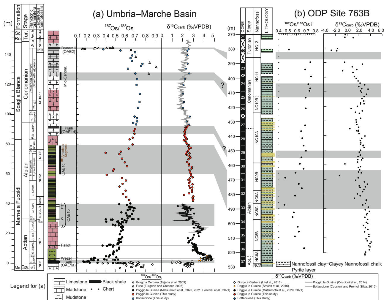
Fig. 2 ^{187}\text{O}/^{188}\text{Os}_i and \delta^{13}\text{C}_{\text{carb}} records of the Umbria-Marche Basin and ODP Site 763B. a Umbria-Marche Basin: lithology, biostratigraphy, and geochemical data are from Coccioni et al. 8,12 , Coccioni and Premoli Silva 9 , Coccioni 65 , Turgeon and Creaser 19 , Tejada et al. 20 , Li et al. 27 , Savian et al. 28 , Matsumoto et al. 13,16 , Percival et al. 29 , and this study. b ODP Site 763B: lithology, biostratigraphy, and geochemical data are from Haq et al. 30 , Bralower et al. 35 , and this study. Ma. Maiolica, Sc. Ro. Scaglia Rossa, Ba. Barremian, Tur. Turonian, G. Globigerinelloides , apt. aptiensis , L. Leupoldina , fer. ferreolensis , algeria. algerianus , H. Hedbergella , troc. trocoidea , M. Microhedbergella , P. Paraticinella , mini. miniglobularis , reni. renilaevs , T. Ticinella , B. Biticinella , Ps. Pseudothalmaninella , su. subticinensis , ticine. ticinensis , Pth. Parathalmaninella , appen. appenninica , Th. Thalmaninella , R. Rotalipora , r. reicheli , g. globotruncanoides , W. Whiteinella , a. archaeocretacea , Hv. Helvetoglobotruncana , h. Helvetica , J. Jacob , K. Kilian , U. Urbino , L. Leenhardt .
