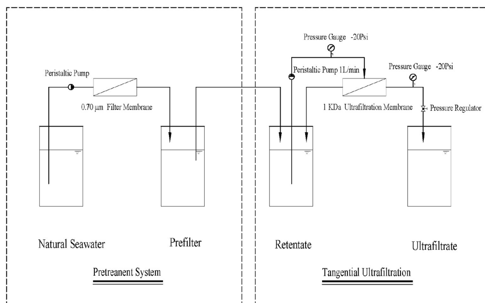
FIGURE 2 | Scheme of the nano-organic carbon (NOC) extraction and separation process.
