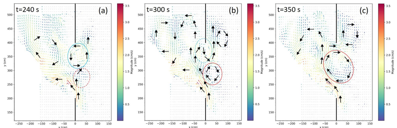
Figure 7. Snapshots of the current velocity field (in cm\ s^{-1} ) at t = 240 s (a), t = 300 s (b) and t = 350 s (c) for Q = 2 and a rotation period T = 60 s (see the black dots in Fig. 5a, the u -field along the black dashed lines in Fig. 6b and Supplementary Figure S6 for the u -profiles along the gap).
