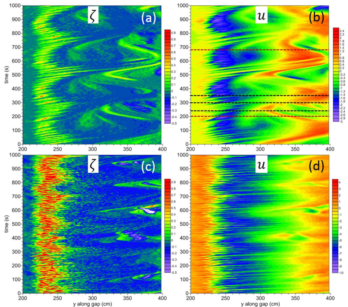
Figure 6. Hovmöller diagram of the relative vorticity \zeta (in s^{-1} )—panel (a)—and current velocity u (in cm\ s^{-1} )—panel (b)—for a rotation period T = 60 s and Q = 2 . Panels (c,d): same but with Q = 8 . The velocity profiles of u along the black dashed lines in panel (b) are shown in the Supplementary Figure S6 and the corresponding snapshots of the 2D u -field are shown in Fig. 7. The brown dashed lines in panel (b) correspond to the snapshots of Fig. 8b,c.
