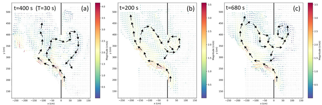
Figure 8. (a) Snapshot of the current velocity field (in \text{cm s}^{-1} ) at t = 400 s for Q = 2 and T = 30 s (cf. Supplementary Figures S3–S5). (b,c) same but for T = 60 s at t = 200 s and at t = 680 s, respectively.
