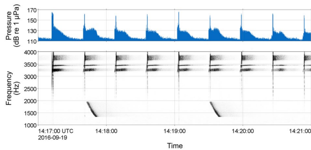
Figure 4. Timeseries (above) and spectrogram (below) displaying a sequence of sonar signals recorded over a 4-min period on September 19th 2016 at Station 5.
