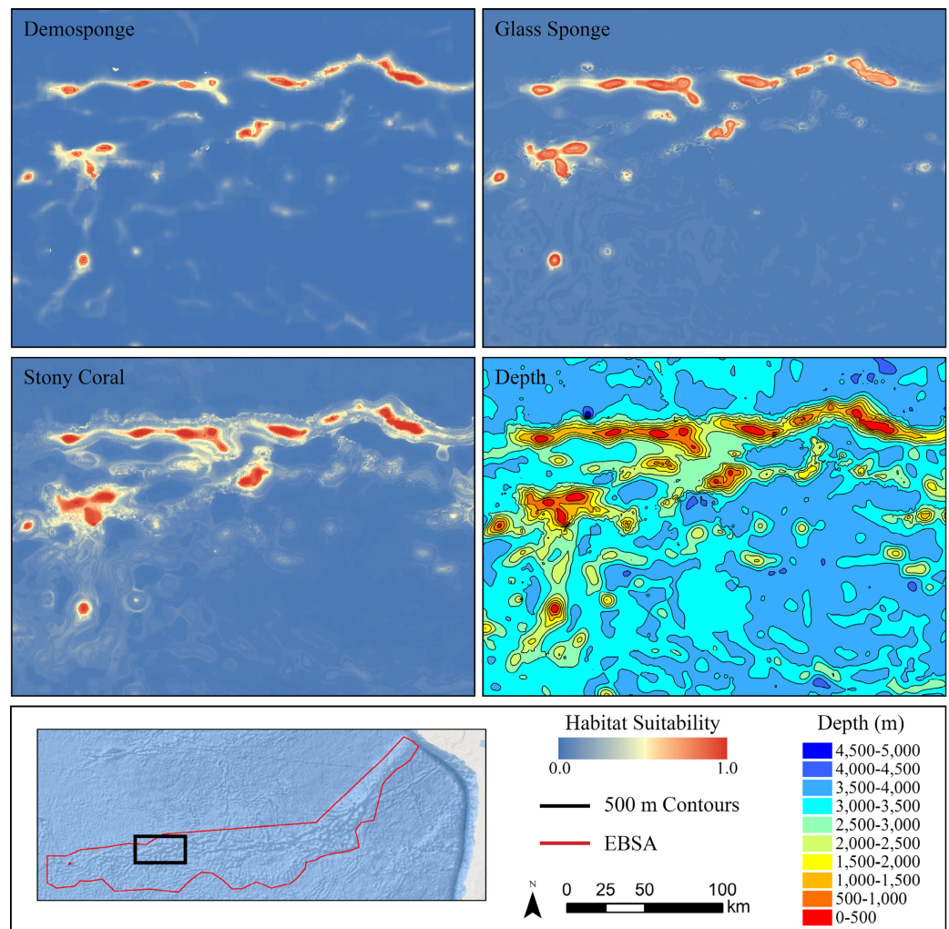
Figure 6 Ensemble models for demosponges, glass sponges, and stony corals showing a subset of highly suitable seamounts on the western side of the Salas y Gómez Ridge. Depth with 500 m contours is shown in the last panel for reference. Full-size DOI: 10.7717/peerj.11972/fig-6
