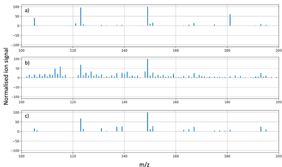
Fig. A.2. Fingerprinting PET nanoplastics in a sample (match confidence ****, z-score > 4), a) Ions in PET library, b) Mass spectra of the surface snow sample (2017-02-28), c) PET nanoplastics signal in the sample (2017-02-28). The signals are normalised to the highest peak. The fingerprint algorithm, scoring and evaluation were in details addressed in our previous work (Materić et al., 2020).
