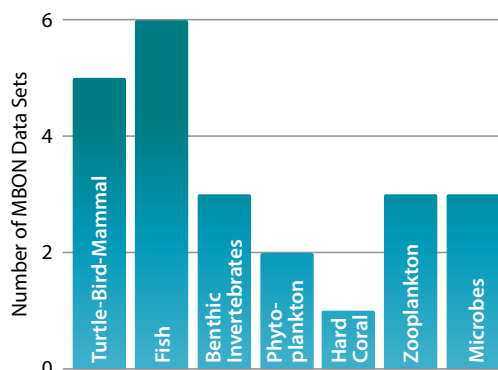
FIGURE 4. MBON managed and collected data contribute to the Global Ocean Observing System Essential Ocean Variables (EOVs) identified by the marine biological community as the most important variables that need to be measured to understand changes in ocean biology and ecosystems. MBON data contribute to this enterprise by making accessible new and legacy data necessary for understanding the status and trends of the EOVs.
