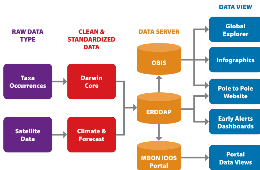
FIGURE 2. Starting from the left of the diagram above, raw data of different types are cleaned, standardized, hosted, and made into data products for end users. On the right are data-driven products designed to address specific user stories from MBON end users. The Global Explorer was developed to display a global map of biodiversity status indicators for each regional Exclusive Economic Zone. The Climate and Forecast standard ( https://cfconventions.org/ ) is most often used with physical oceanographic data and the Network Common Data Form (NetCDF) format. OBIS = Ocean Biodiversity Information System. IOOS = Integrated Ocean Observing System.
