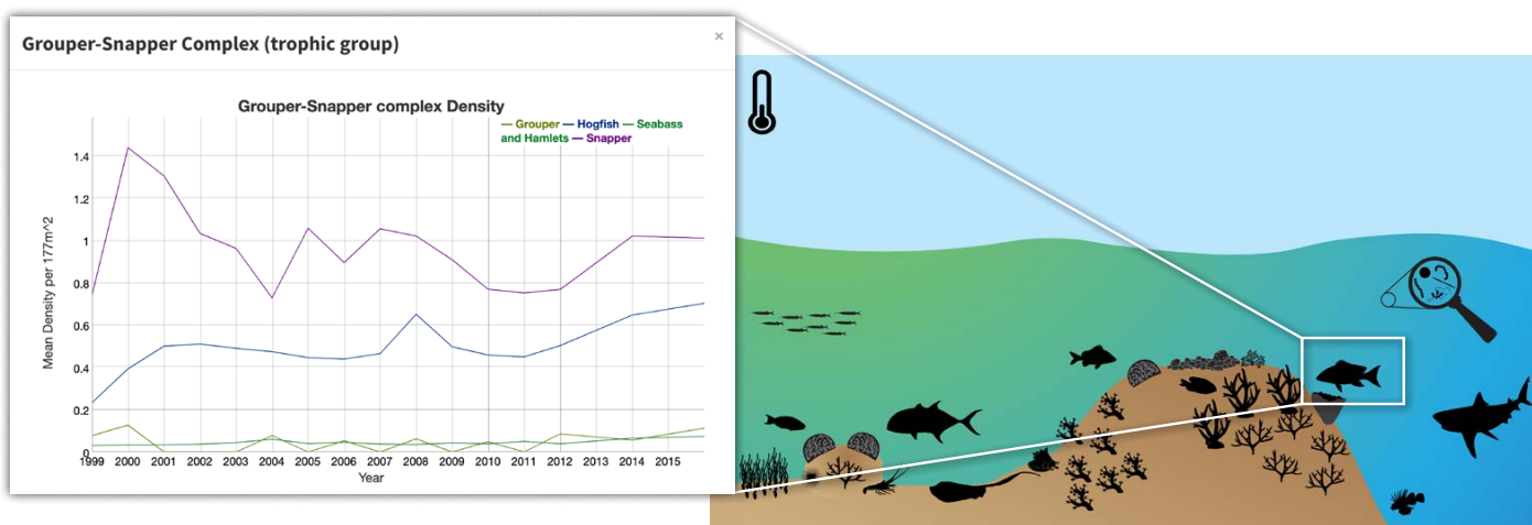
FIGURE 6. NOAA Southeast Fisheries Science Center reef visual census monitoring data are incorporated here into a Florida Keys National Marine Sanctuary interactive infographic for exploring status and trends of different biological variables.
