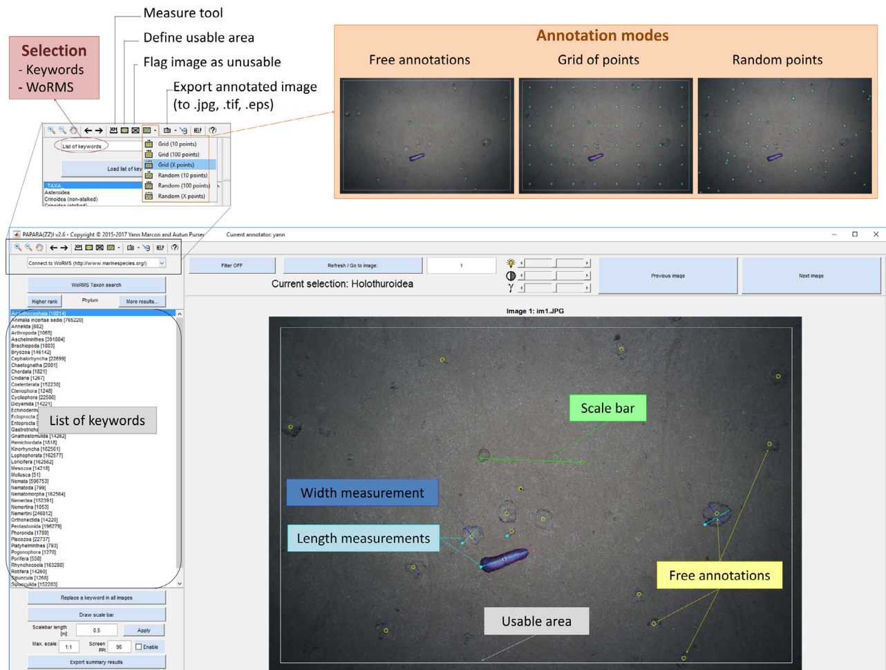
Fig. 5. View of the main annotation graphical interface of PAPARA(ZZ)I . Most of the functionalities can be called directly from this interface. The image shows free annotations (yellow circles), length/width measurements (light/dark blue lines), a scale bar (green line) and the boundary of the useable area (white rectangle). (For interpretation of the references to colour in this figure legend, the reader is referred to the web version of this article.)
