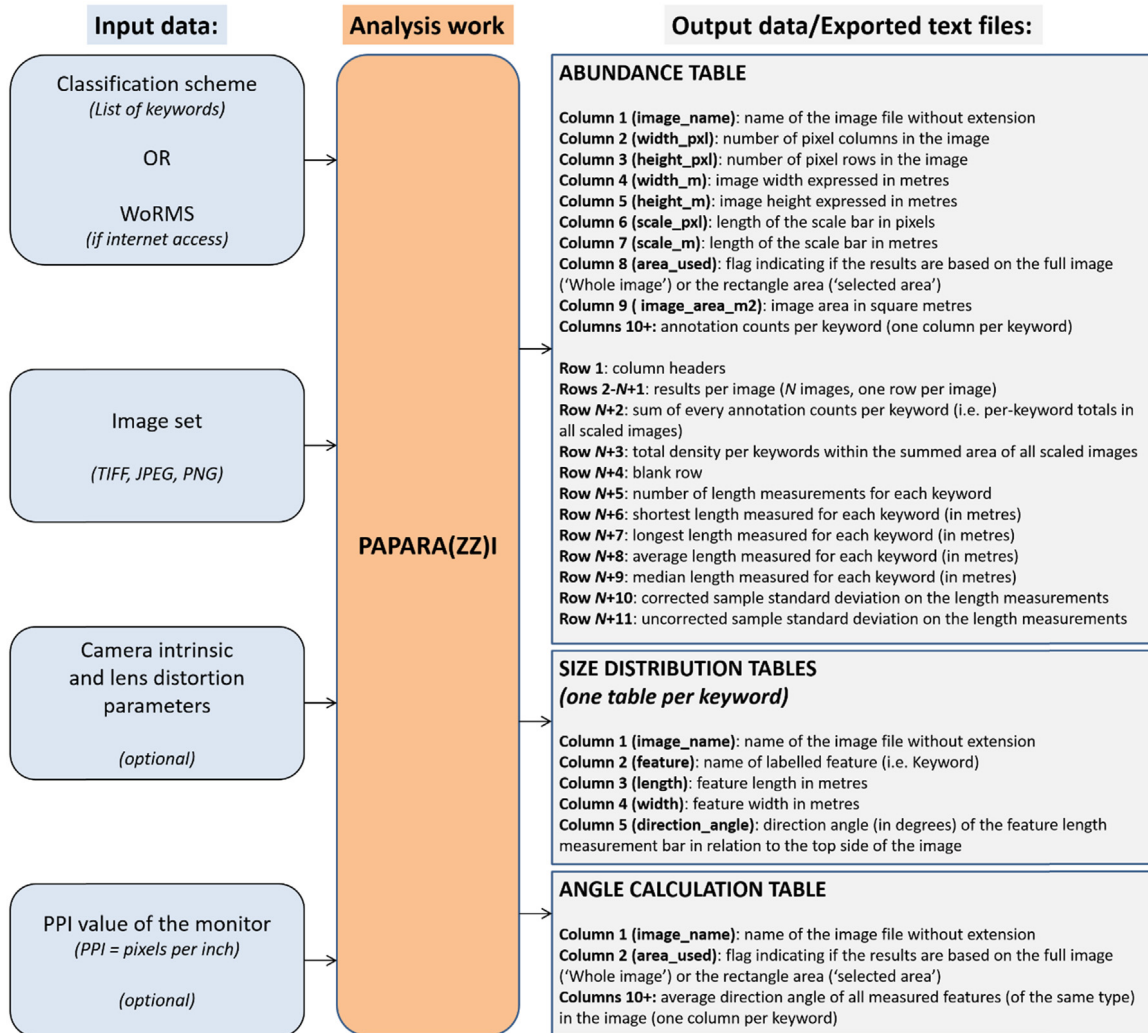
Fig. 2. Flow chart describing the PPARA(ZZ)I inputs and outputs. Apart from the set of images to analyse, PPARA(ZZ)I only requires a list of keywords to be provided. All other inputs are optional. Output data are stored as tables within text files with a simple structure. The structure of the output files is described. The structure of the output files is the same for all annotation modes (free points, point grid, random points).
